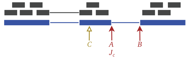
(A) An example of a normally spliced transcript, assuming Veridical is validating a specific variant, C, shown in yellow. The adjacent intron-exon boundary, in this case, corresponds to both the adjacent splice junction, J_c and the relevant natural site A. B is the downstream natural site. Veridical would not identify any aberrant splicing.
