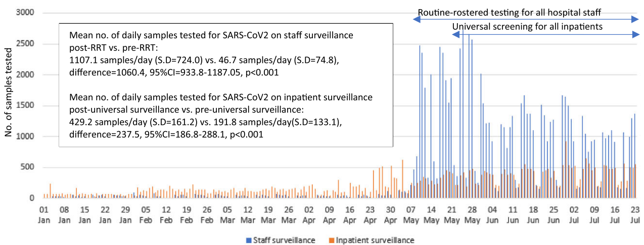
Fig. 1. a: Map of community clusters in proximity to the hospital campus of a large Singaporean tertiary hospital. b: Timeline of COVID-19 outbreak in neighbouring community, and detection of COVID-19 cases amongst staff and patients through hospital surveillance. c: Volume of SARS-CoV-2 testing (PCR) for staff and patients at a large Singaporean tertiary hospital.
