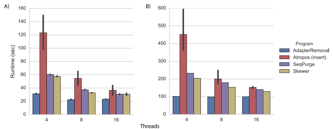
Figure 3 Trimming execution time for real data. Execution time on (A) WGBS and (B) mRNA-Seq datasets for programs running on a cluster node with 4, 8, and 16 threads. Each program was executed multiple times, and Atropos was run with the insert-match algorithm and parallel-write output mode. The mean execution times for each program are shown with 95% CI.
