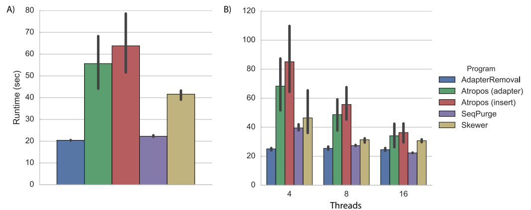
Figure 2 Trimming execution time for simulated data. Execution time on simulated datasets for programs running on (A) a desktop computer with four parallel processes (threads), and (B) a cluster node with 4, 8, and 16 threads. Each program was executed multiple times, and Atropos was run with combinations of alignment algorithm (insert-match or adapter-match) and output mode (worker-compression, writer-compression, or parallel-write). The mean execution times for each program are shown with 95% CI.
