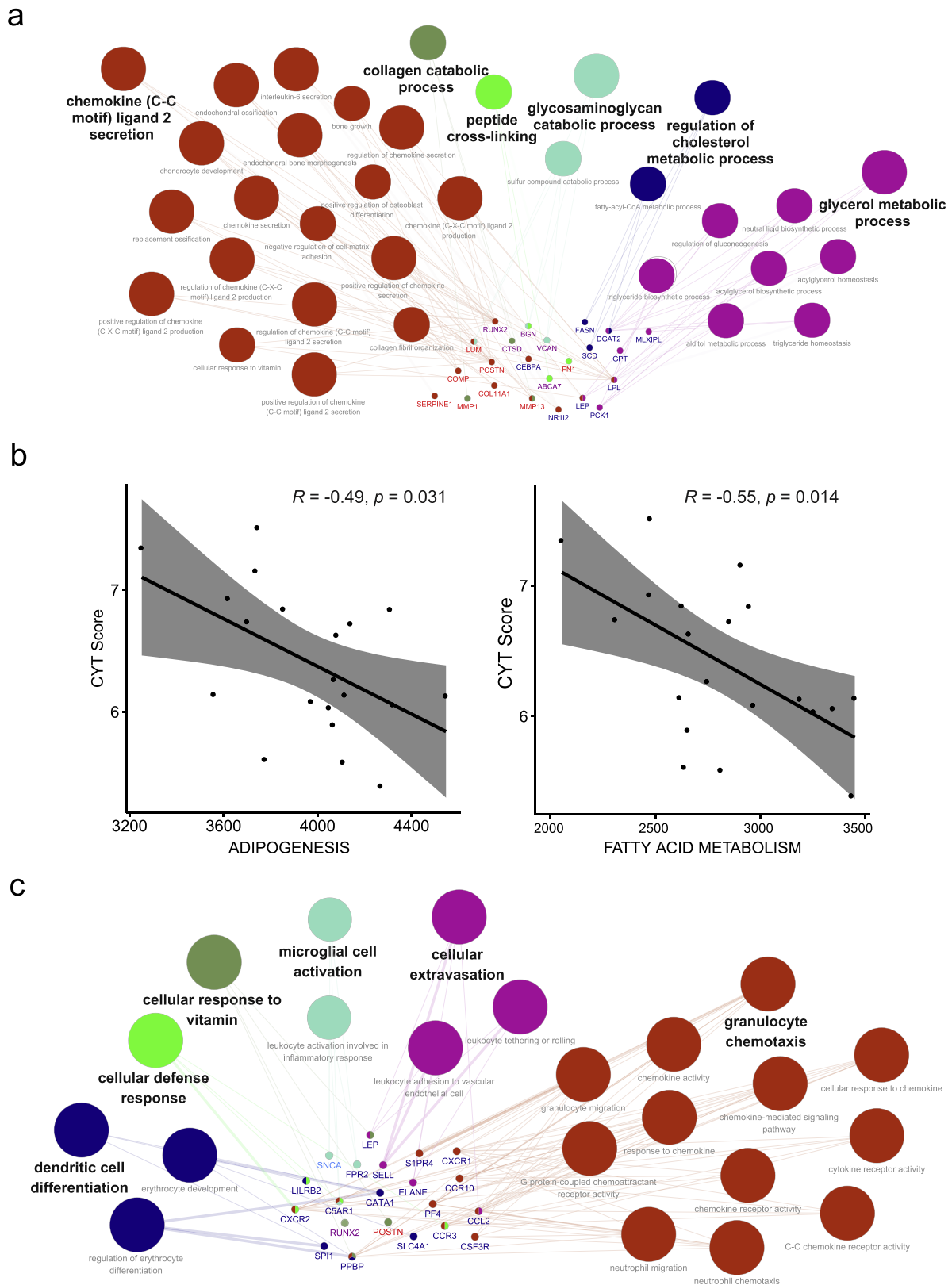
Fig. 3. . PPI network and Hubgene analysis. A. Hubgenes were selected from the DEGs and IS genes from immune-hot MEC tumor intrinsic analysis. Genes were grouped into functionally similar GO terms. The size of GO term indicates the number of genes matched to the term, with the greater number of gene being larger. Colors of genes represent the following: Red: DE up; Violet: IS up; Blue: DE down; Sky blue: IS down. B. Correlation between GSEA identified significantly enriched 'Hallmark fatty acid metabolism' and 'Hallmark adipogenesis' with CTY score. C. Immune-cold MEC tumor intrinsic analysis. Genes were grouped into functionally similar GO terms. The size of GO term indicates the number of genes matched to the term, with the greater number of genes being larger. Colors of genes represent: Red: DE up; Violet: IS up; Blue: DE down; Sky blue: IS down. Statistics in A and C: GO term analysis. All q -values for significance < 0.05 and significant fold change (FDR < 0.01 ). R values represent the Pearson correlation coefficients.
