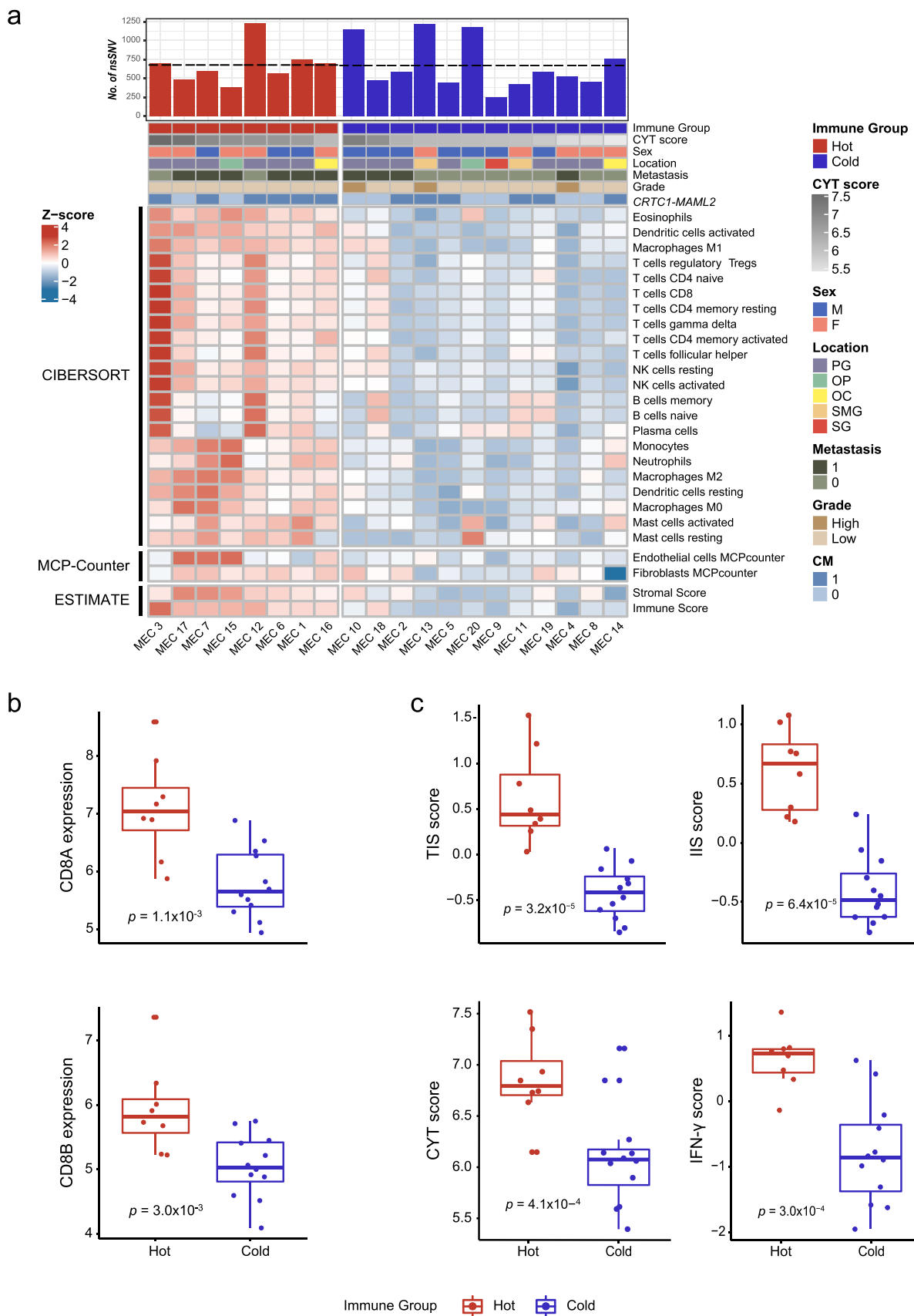
Fig. 1. Comprehensive immune landscape and immune modulator illustration representing immune subtypes of MEC. A. Single-sample genaset enrichment analysis (ssGSEA) of 20 patients with MEC identified two immunophenotypically distinctive subgroups based on different immune and stromal cell-infiltration levels. Top bar plot represents the number of gene mutations in each sample. B. Comparison of CD8A and CD8B expression between the immune-hot and -cold MEC. C. Comparison of the TIS, IIS, INFG, CYT, and APM scores between the immune-hot and -cold MEC. Statistics in A–C: Wilcoxon test. All P -values for significance < 0.05.
