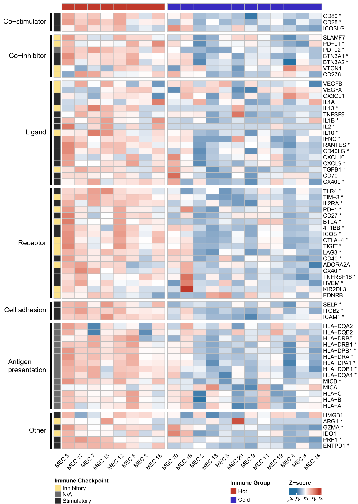
Fig. 2. Comparison of immunomodulator genes between the two immune MEC subgroups. Comparison of immune modulatory regulator genes between the immune-hot and -cold MEC. Statistics: Wilcoxon test. P-values for significance < 0.05.
