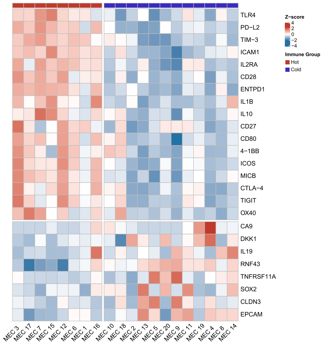
Fig. 4. . Comparison of PD-1, PD-L1, and immuno-oncological (IO) target gene expression difference between the two immune MEC subgroups. A. Comparison of PD-1 and PD-L1 score between the immune-hot and -cold MEC subgroups. B. Heatmap showing expression of immuno-oncological therapeutic target genes between the immune-hot and -cold MEC subgroups. Upper part shows target genes that are differentially upregulated in the immune-hot MEC, and lower part shows target genes that are differentially upregulated in the immune-cold MEC. Statistics in A: Wilcoxon test. All P-values for significance < 0.05.
