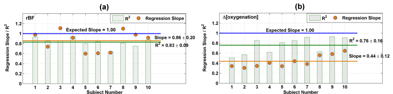
Figure 4 | Regression slopes and correlation coefficients between the contact and noncontact measurements in rBF (a) and \Delta[oxygenation] (b) for the ten subjects.
