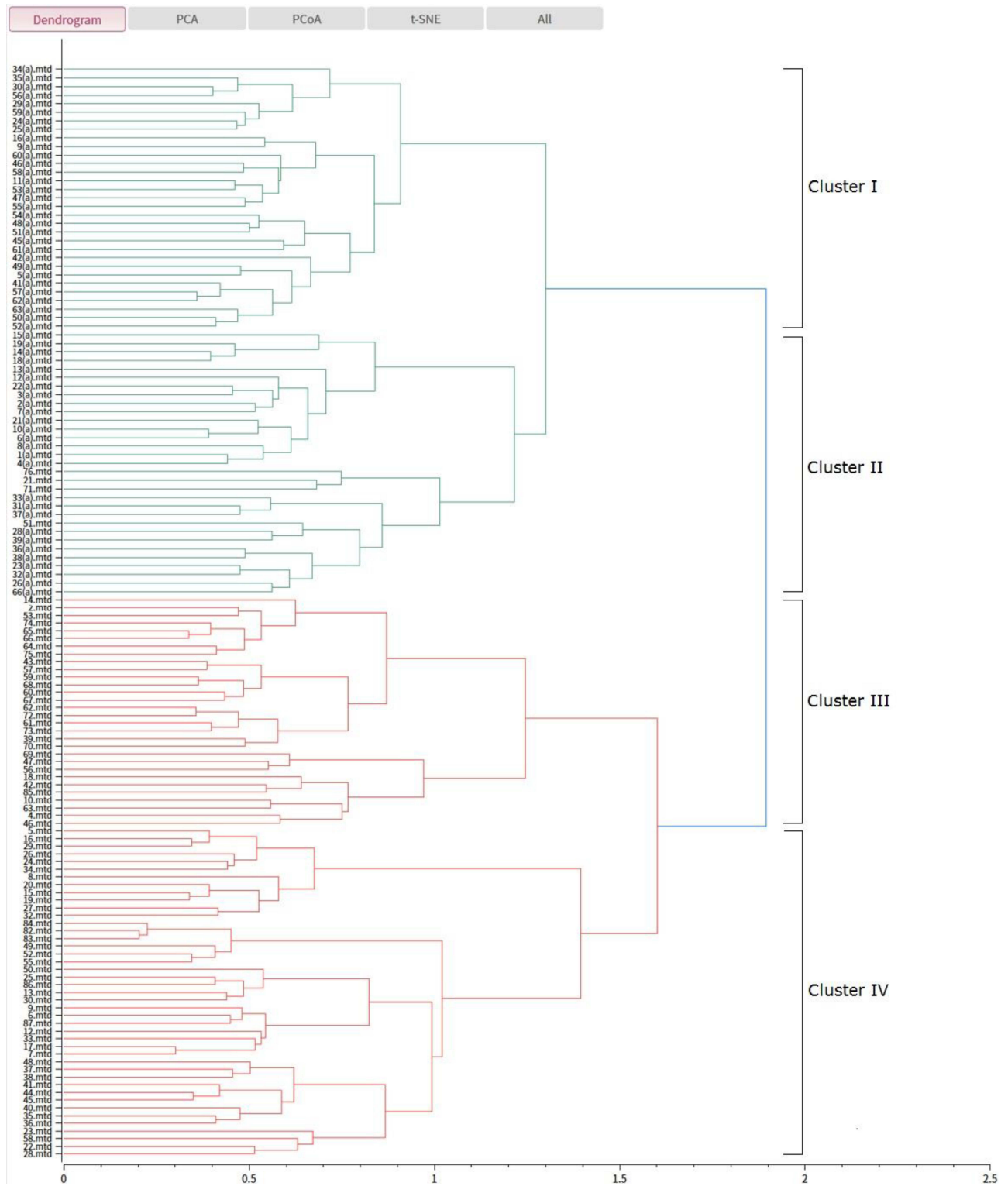
Figure 2 Hierarchical clustering of Talaromyces marneffii isolates by MALDI-TOF MS. The hierarchical clustering of MALDI-TOF peak profiles identified four different clusters. All T. marneffii strains, except for strain 5, from HIV-negative patients belonged to cluster II in Fujian, which were different in Guangxi. The strains of non-HIV-infected patients were in cluster III and IV in Guangxi.
