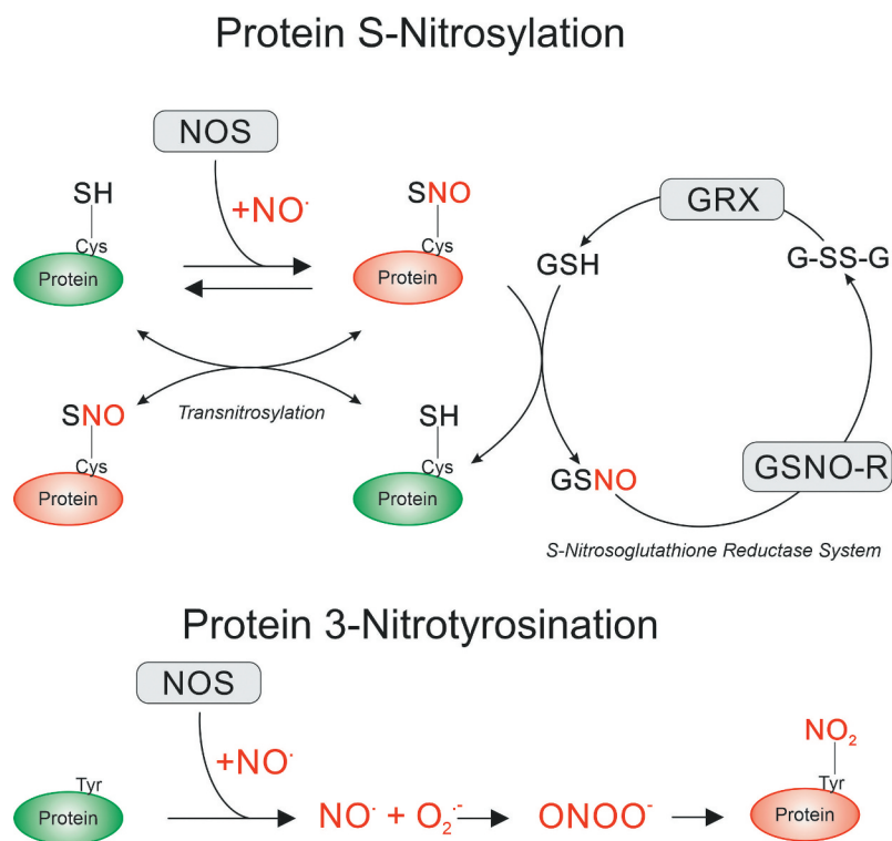
Figure 1. Post-translational modifications mediated by NO signaling. NO produced by nitric oxide synthases (NOS) can directly attack protein cysteine side chains to induce S-nitrosylation (SNO). This is a reversible modification that can be transferred to other protein cysteine side chains (transnitrosylation) or reduced by glutathione (GSH) to the native protein via the S-Nitroso-glutathione reductase (GSNO-R) system. The S-Nitroso-glutathione (GSNO) formed is then recycled via GSNO-R to oxidized GSH (GSSG) for further reduction to GSH by glutaredoxins (GRX). NOS-derived NO can also irreversibly attack tyrosine residues via the intermediate production of NO, superoxide radical ( \text{O}_2^- ), and peroxynitrite ( \text{ONOO}^- ), forming 3-Nitrotyrosine modified proteins.
