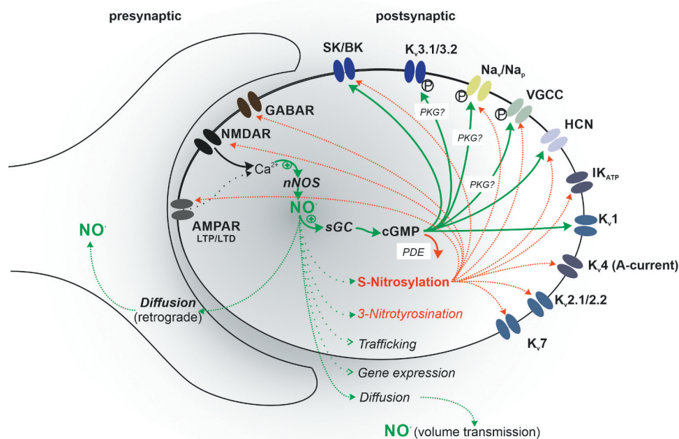
Figure 2. Schematic overview of ion channel modulation by S-nitrosylation and cGMP-dependent mechanisms. Several ion channel families are modulated by redox-sensitive mechanisms including S-nitrosylation. Other channel families are modified by both redox-sensitive and direct cGMP-dependent signaling (in addition to protein kinase G (PKG) activation with subsequent protein phosphorylation). A combination of the above signaling and modulation of different or multiple residues within one channel protein may lead to graded or opposing effects on channel conductances or kinetics with diverse outcomes for neuronal excitabilities. These complex modulatory effects depend on the redox state on the cell, amount of available NO and activities of mechanisms, which reverse the signaling, such as de-/trans-nitrosylation, breakdown of cGMP via phosphodiesterases (PDE), or dephosphorylation by phosphatases.
