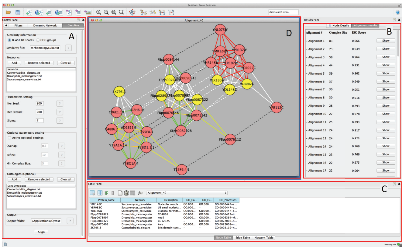
Figure 1. GASOLINE Cytoscape panels: A) GASOLINE parameters; B) Alignment results; C) Description of selected proteins and associated GO terms; D) Alignment visualization: intra-edges are represented with solid lines and coloured according to their weight (green for low values, yellow for medium values and red for high values); inter-edges are drawn with dashed lines.
