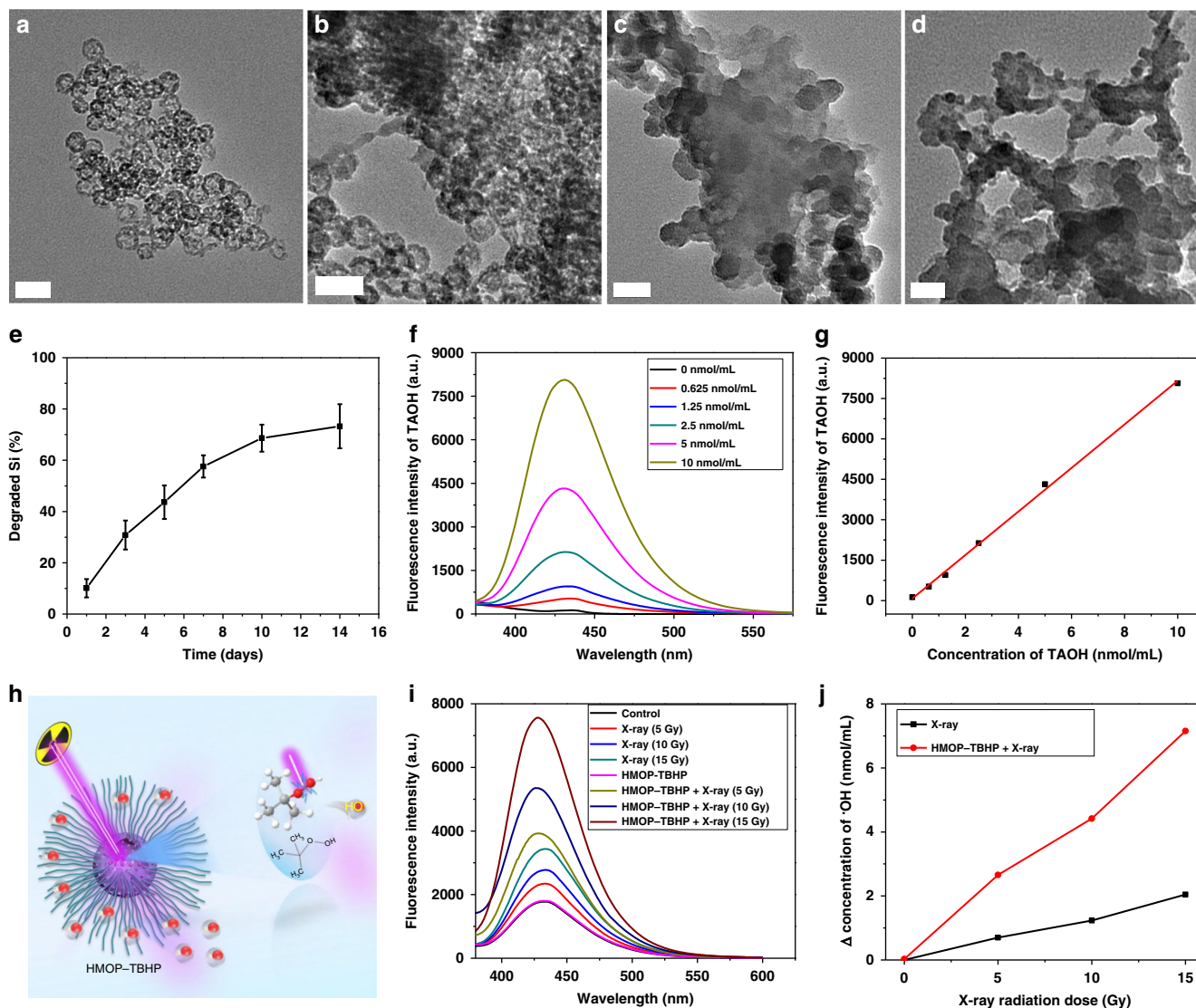
Fig. 4 Biodegradation of HMOP and X-ray-activated \bullet\text{OH} generation. a–d TEM images of thioether-hybridized HMOP dispersed in PBS with 10 mM GSH for 1 day ( a ), 3 days ( b ), 7 days ( c ), and 14 days ( d ). Scale bar: 50 nm. e Degradation curve of thioether-hybridized HMOP in PBS with 10 mM GSH within 14 days. n = 3 , mean \pm s.d. f Fluorescence emission spectra of TAOH with different concentrations. g Standard curve for the linear relation between the concentration of TAOH and its fluorescence intensity at \lambda = 430 nm. h Schematic of X-ray-activated cleavage of peroxy bond within TBHP (encapsulated in the cavity of HMOP) for generation of \bullet\text{OH} . i Fluorescence spectra of TAOH (oxidized TA) subjected to varied doses (0, 2, 4, 6 Gy) of X-ray irradiation with or without HMOP-TBHP. j The \bullet\text{OH} concentrations calculated by \bullet\text{OH} -triggered oxidation of TA into 2-hydroxyterephthalic acid (TAOH)
