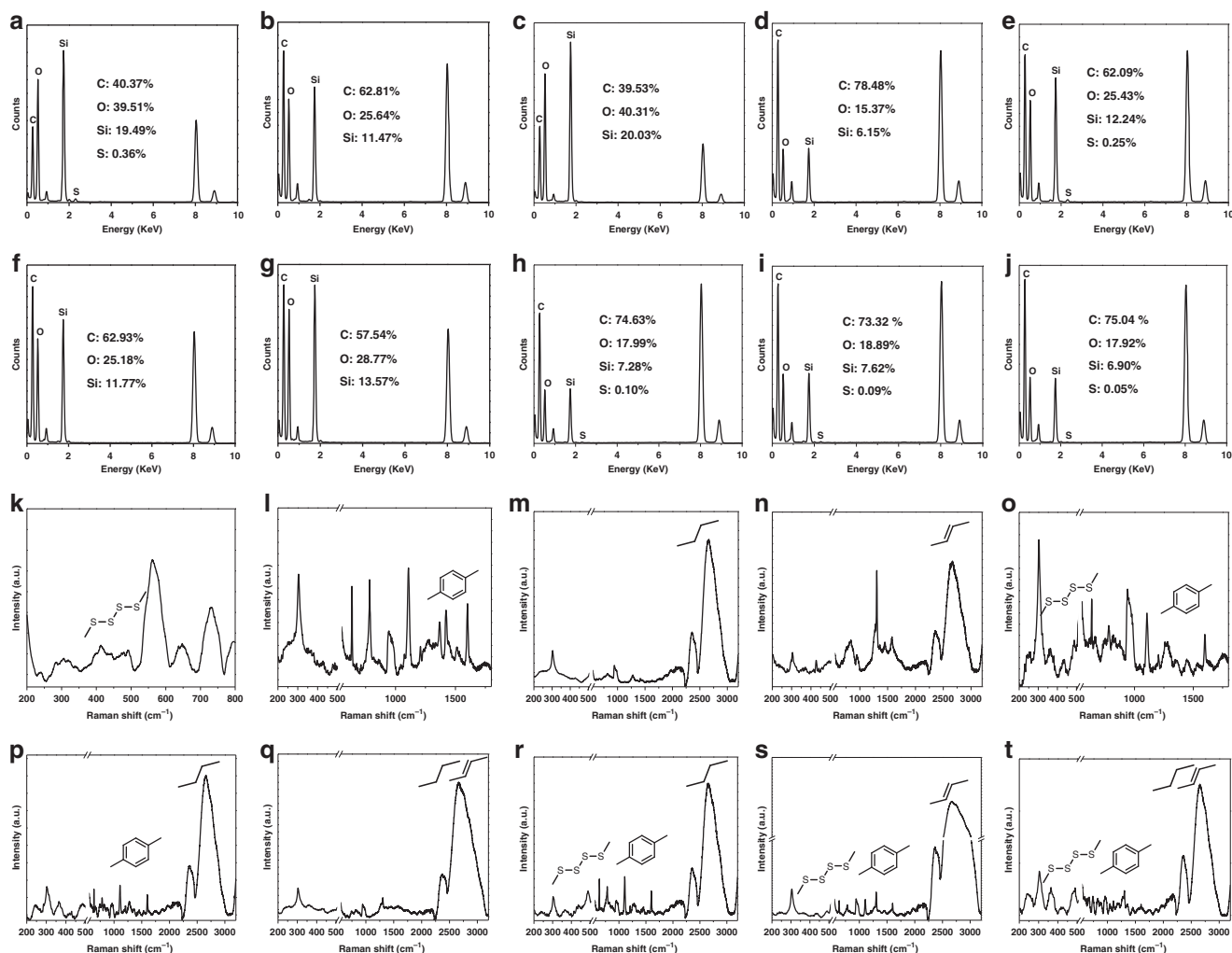
Fig. 3 Elemental analysis and Raman spectra of multiple small-sized HMOPs. Energy-dispersive X-ray spectroscopy (EDS) spectra (a–j) and Raman spectra (k–t) of sub-50 nm HMOPs with framework hybridization of different organic moieties. Mono hybridization: thioether (a, k), phenylene (b, l), ethane (c, m), ethylene (d, n). Double hybridization: thioether/phenylene (e, o), phenylene/ethane (f, p), ethane/ethylene (g, q). Triple hybridization: thioether/phenylene/ethane (h, r), thioether/phenylene/ethylene (i, s). Quadruple hybridization: thioether/phenylene/ethane/ethylene (j, t). Inset in a–j: The atomic percentages of the major elements are presented in each EDS spectrum of small-sized HMOP. Inset in k–t: The representative moieties are presented in each Raman spectrum of small-sized HMOP
