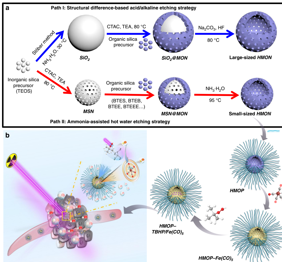
Fig. 1 Synthesis and biomedical application of HMOP-TBHP/ \text{Fe}(\text{CO})_5 . a Schematic of the different synthetic paths for large-sized HMON and small-sized HMON through a structural difference-based acid/alkaline etching strategy and an ammonia-assisted hot water etching strategy, respectively. Herein, a versatile method is first proposed for the generic synthesis of a library of sub-50 nm HMONs with multiple framework hybridization of diverse organic moieties by changing only the introduced bisilylated organosilica precursors. b Schematic of the construction of HMOP-TBHP/ \text{Fe}(\text{CO})_5 for X-ray-activated synergistic radiodynamic/gas therapy. Through PEGylation and co-delivery of TBHP/ \text{Fe}(\text{CO})_5 by taking advantage of the hollow mesoporous structure of HMON, the cascaded generation of \cdot\text{OH} and CO molecules based on the X-ray-activated sequential bond cleavage will give rise to synergistic radiodynamic/gas therapy with extremely little oxygen reliance, thus overcoming the Achilles' heel of conventional radiotherapy
