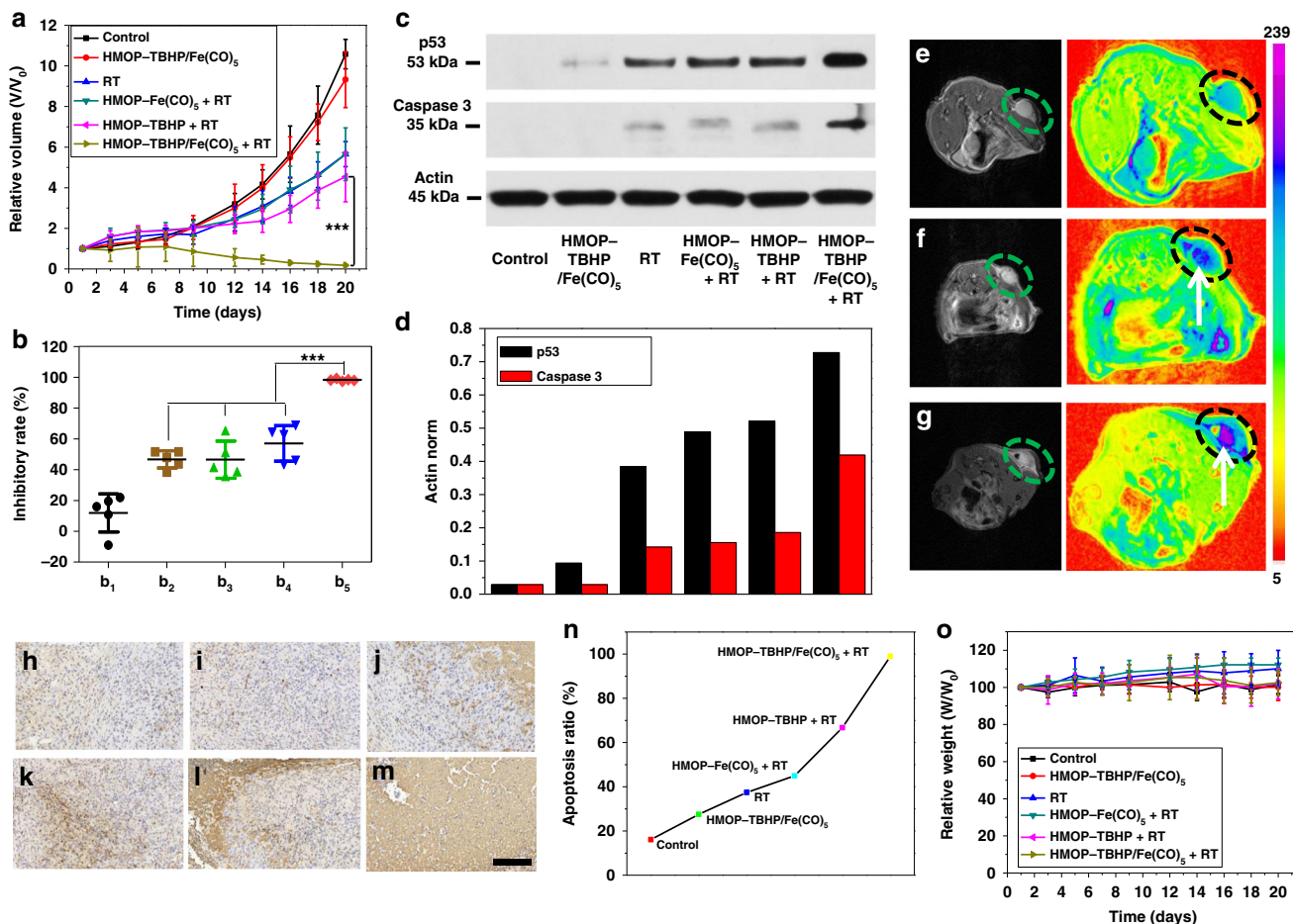
Fig. 9 In vivo evaluation of synergistic RDT/gas therapy. a U87MG tumor growth curves after different treatments. b Inhibitory rates of U87MG tumors at day 20 post treatment: HMOP-TBHP/Fe(CO) 5 (b 1 ), RT (b 2 ), HMOP-Fe(CO) 5 + RT (b 3 ), HMOP-TBHP + RT (b 4 ), HMOP-TBHP/Fe(CO) 5 + RT (b 5 ). n = 5, mean ± s.d., *** P < 0.001, Student's two-tailed t -test. c Western blot analysis of p53 and caspase 3 expression in U87MG tumors after different treatments. Uncropped image available in Supplementary Fig. 44. d The corresponding quantitative analysis of p53 and caspase 3 expression in c . e–g T 2 -weighted MR imaging and the corresponding pseudo-color images of U87MG tumors at day 3 post treatment: control ( e ), RT ( f ), HMOP-TBHP/Fe(CO) 5 + RT ( g ). The white arrows refer to the apoptotic area in tumor. h–m TUNEL-stained sections of U87MG tumors subjected to different treatments: control ( h ), HMOP-TBHP/Fe(CO) 5 ( i ), RT ( j ), HMOP-Fe(CO) 5 + RT ( k ), HMOP-TBHP + RT ( l ), HMOP-TBHP/Fe(CO) 5 + RT ( m ). n = 5 sections per group. Scale bar: 200 μm. n Quantitative analysis of tumor cell apoptosis in h–m by using the Image-pro plus 6.0 software (Media Cybernetics, Inc., MD, USA). o Weight change curves of U87MG tumor-bearing mice after different treatments. n = 5, mean ± s.d.
