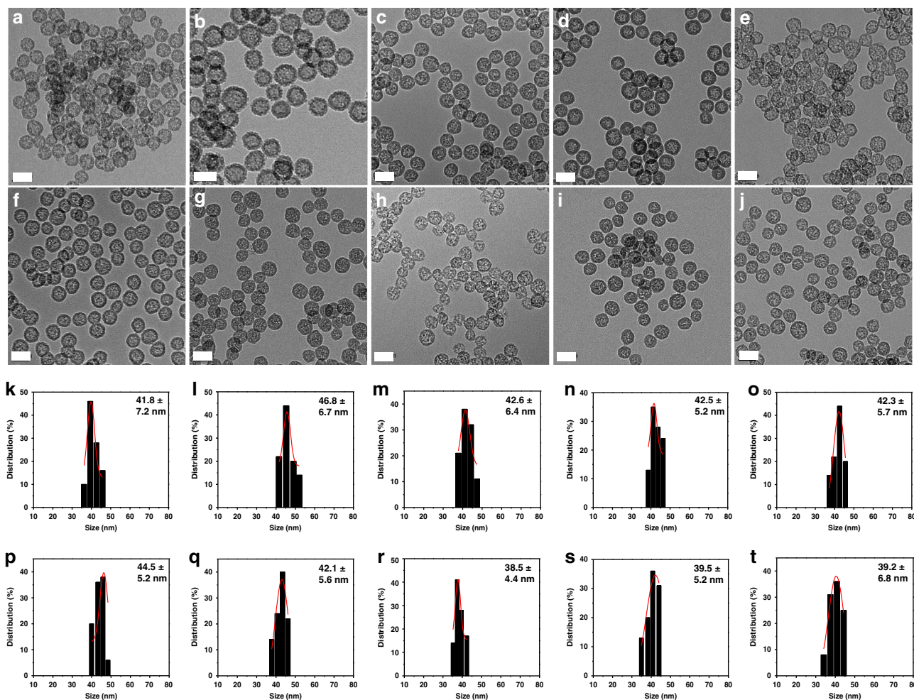
Fig. 2 Morphology and size distributions of multiple small-sized HMONS. TEM images ( a–j ) and size distributions ( k–t ) of sub-50 nm HMONS with multiple framework hybridization of diverse organic moieties. Mono hybridization: thioether ( a, k ), phenylene ( b, l ), ethane ( c, m ), ethylene ( d, n ). Double hybridization: thioether/phenylene ( e, o ), phenylene/ethane ( f, p ), ethane/ethylene ( g, q ). Triple hybridization: thioether/phenylene/ethane ( h, r ), thioether/phenylene/ethylene ( i, s ). Quadruple hybridization: thioether/phenylene/ethane/ethylene ( j, t ). Scale bar: 50 nm. Despite different framework hybridization, the as-synthesized HMONS demonstrate a uniform hollow-structured spherical morphology with size below 50 nm, which confirms the advantage of this well-established ammonia-assisted hot water etching strategy in the generic synthesis of a library of small-sized HMONS
