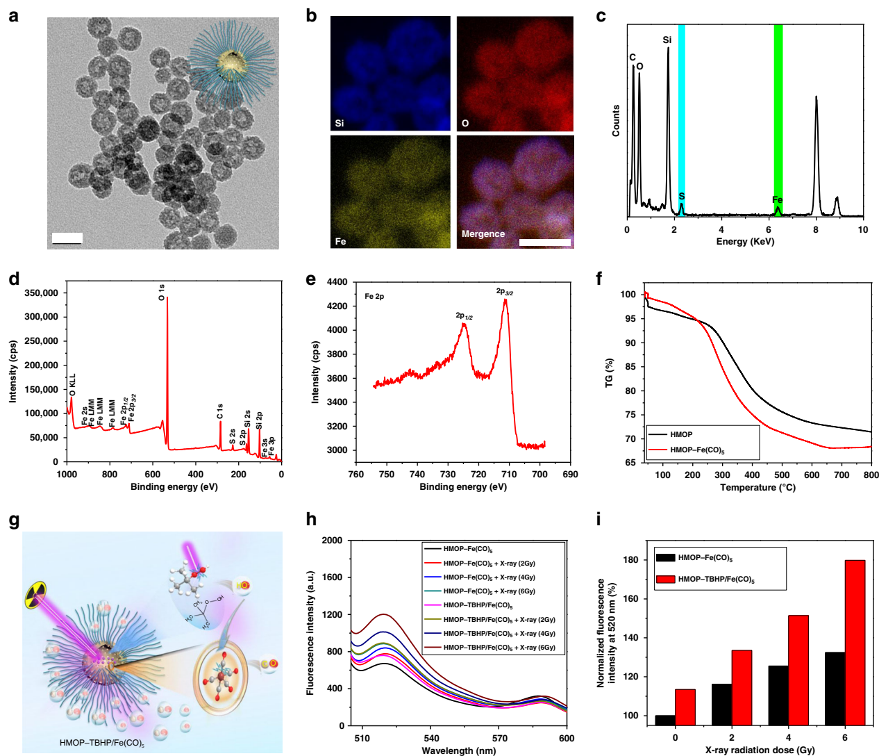
Fig. 6 Construction of HMOP-TBHP/Fe(CO) 5 and X-ray-activated CO release. a TEM image of HMOP-Fe(CO) 5 . Scale bar: 50 nm. b Elemental mapping (Si, O, Fe) of HMOP-Fe(CO) 5 . Scale bar: 50 nm. c EDS spectrum of HMOP-Fe(CO) 5 . d X-ray photoelectron spectroscopy (XPS) spectrum of HMOP-Fe(CO) 5 . e Binding energies of Fe(2P 3/2 ) and Fe(2P 1/2 ) correspond to 711 and 724 eV, respectively, indicating the attachment of Fe(CO) 5 to HMOP. f Thermo-gravimetric (TG) curves of HMOP and HMOP-Fe(CO) 5 . g Schematic of X-ray-triggered CO release from HMOP-TBHP/Fe(CO) 5 . h Fluorescence spectra of COP-1 probe subjected to varied doses (0, 2, 4, and 6 Gy) of X-ray irradiation in the presence of HMOP-Fe(CO) 5 or HMOP-TBHP/Fe(CO) 5 . i Evaluation of CO generation based on the normalized fluorescence intensity of COP-1 probe at 520 nm
