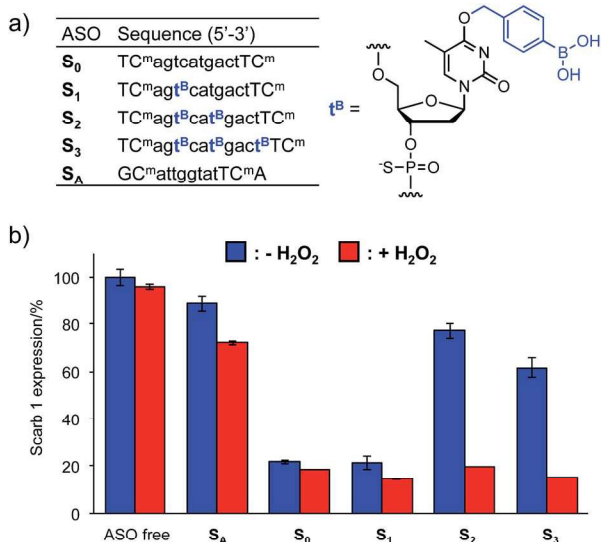
Fig. 4 (a) Sequences of ASOs. n = DNA, N = LNA (C m = LNA-5-Me-cytidine), all internucleosidic linkages are phosphorothioated. (b) Intercellular gene silencing triggered by H 2 O 2 using boronate ASOs. Three independent experiments were averaged and the error bars represent standard deviation.
