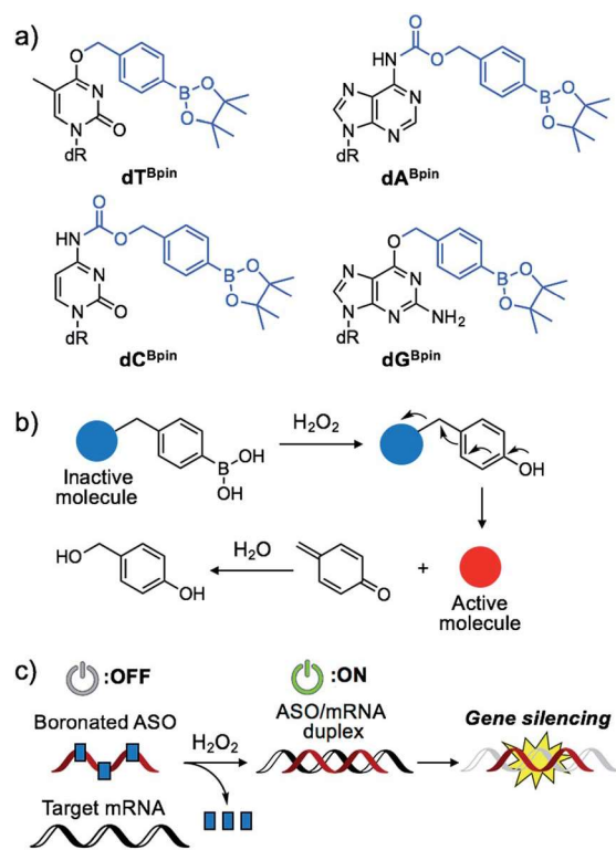
Fig. 1 (a) Chemical structure of boronated 2'-deoxyribonucleoside analogues synthesized in this study. (b) Schematic of \text{H}_2\text{O}_2 -triggered molecule activation. (c) Gene silencing triggered by \text{H}_2\text{O}_2 through inactive boronated ASOs.
