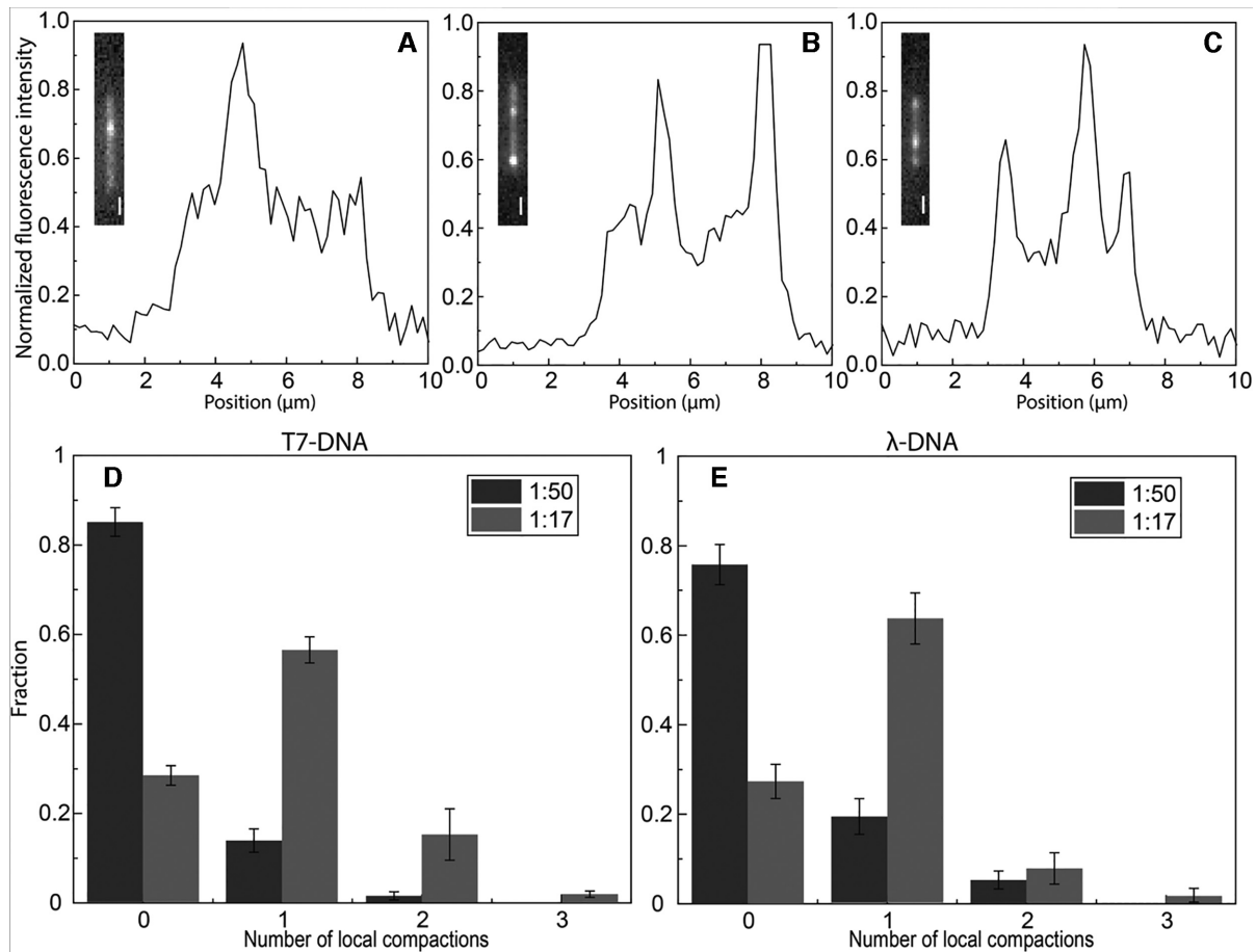
Figure 2. (A–C) Representative intensity profiles of \lambda -DNA with 1 (A), 2 (B) and 3 (C) local condensates. Insets show fluorescence snapshot images of YOYO-1 stained \lambda -DNA with corresponding local condensates. The scale bars are 2 \mu\text{m} . (D, E) Number of local condensates along blunt ended T7-DNA (D), and \lambda -DNA with 12 bp overhangs (E), in the presence of 0.1 \mu\text{M} (black) or 0.3 \mu\text{M} (gray) NC, with 5 \mu\text{M} DNA (in bp). As these concentrations are above K_d , these conditions correspond to 1 NC molecule bound per 50 or 17 bp, respectively, as indicated in panels A and B. Values are expressed as mean \pm SD.
