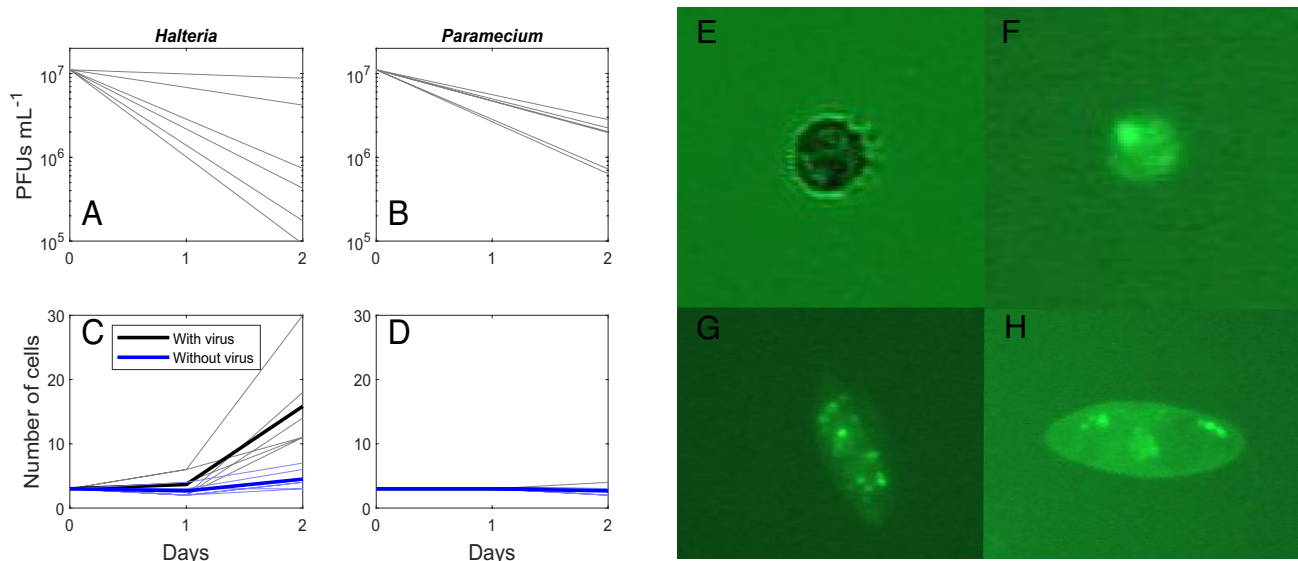
Fig. 1. Halteria (A) and Paramecium bursaria (B) reduced plaque-forming unit density by twofold to two orders of magnitude in 2 d. Supplemental feeding of chloroviruses to the ciliate Halteria led to pronounced growth (C, black lines); in control dishes without virus, Halteria cell abundance was steady (C, blue lines). Paramecium (D) showed no cell growth in response to feeding with viruses. Light solid lines are individual replicates; thick lines are averages. Fluorescent micrographs of ciliates fed chloroviruses show Halteria with visible light (E) and with fluorescently labeled virus given as food (F). Two other ciliates, Euplotes sp. (G) and Paramecium caudatum (H), also show the indication of virus uptake. Aggregations of viruses are visible in the inside of vacuoles.
