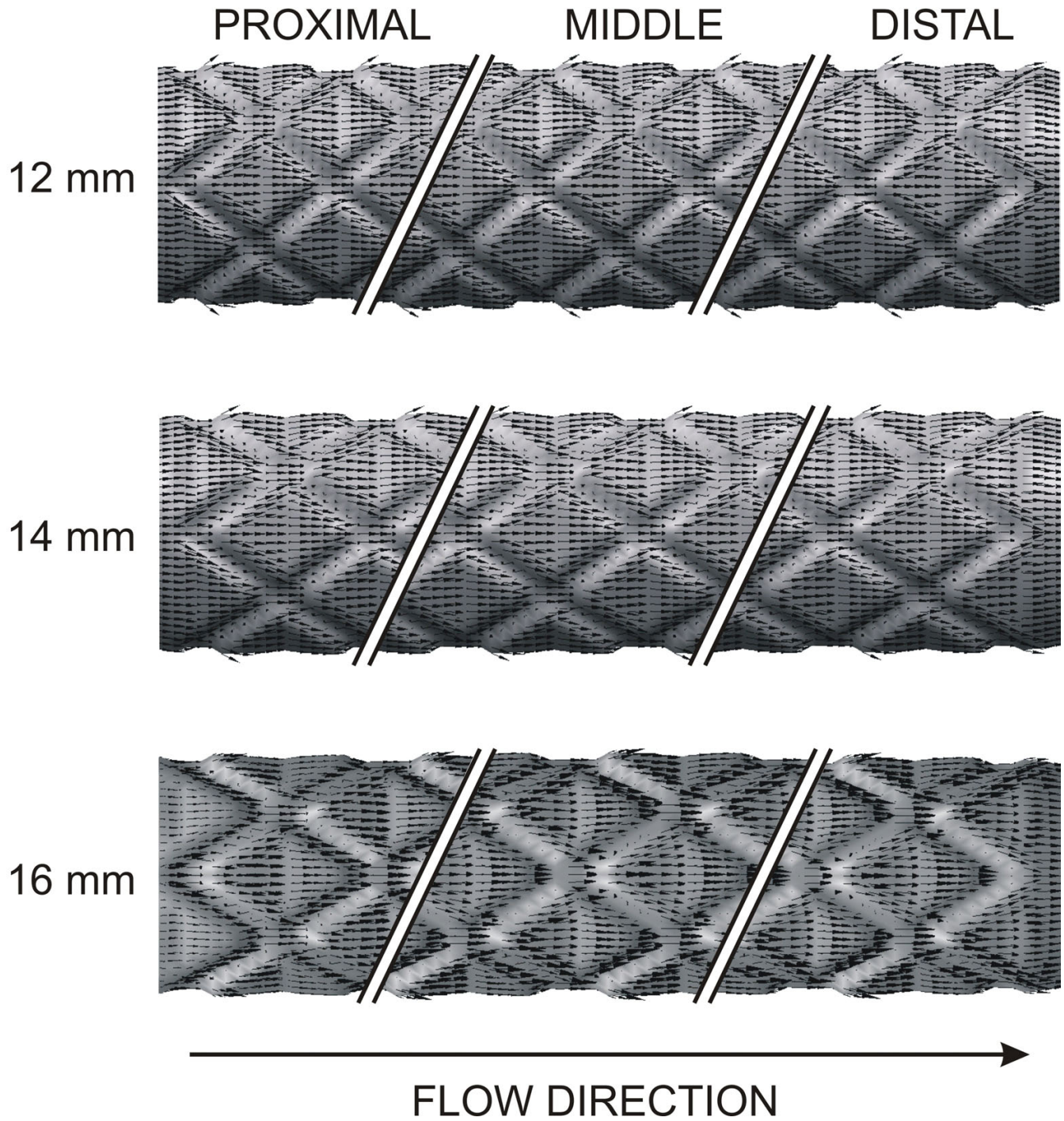
Figure 4 Value-weighted near-wall velocity vectors in the proximal, middle and distal portions of the stent resulting from the unique strut orientation angles corresponding to ideal (16 mm) and progressively foreshortened stents (14 and 12 mm).
