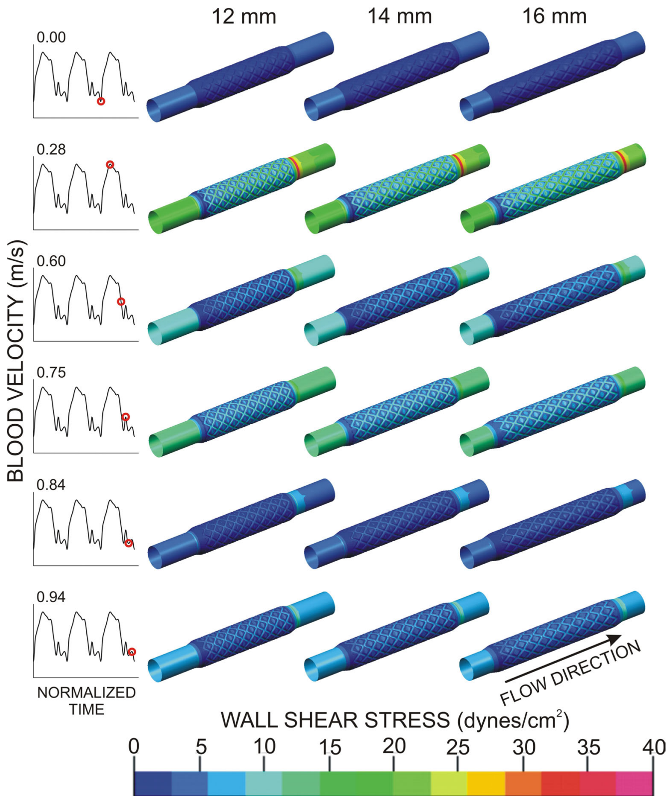
Figure 5 Time-dependent alterations in spatial wall shear stress throughout the cardiac cycle in ideal stents (16 mm) and those with progressive degrees of foreshortening (14 and 12 mm).
