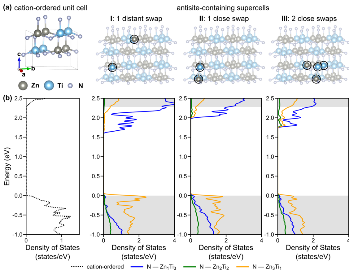
Figure 8. (a) Crystal structures of cation-ordered \text{ZnTiN}_2 and three antisite-containing 128-atom supercells with the exchanged Zn and Ti atoms highlighted. (b) Partial density of states per N-centered tetrahedra for the cation-ordered material and the three supercells, with the contributions from the different N-centered tetrahedra illustrated. Gray shading indicates the band edges from the cation-ordered material. Gaussian smearing is used in our Brillouin zone integrations, using a smearing parameter of 0.03 eV.
