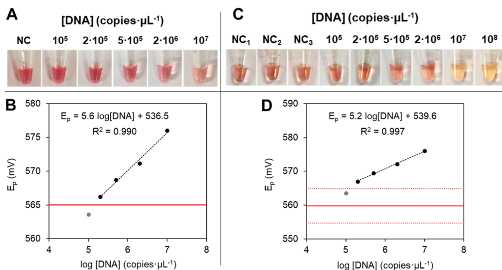
Figure 3. (A) End-point LAMP products obtained using different initial DNA dilutions (copies· \mu\text{L}^{-1} are shown in figure). A negative control (NC) is also shown. (B) Calibration plot using electrochemical LAMP detection for the reactions shown in (A). The peak potential value for NC is represented as a continuous red line. The value for 10 5 copies· \mu\text{L}^{-1} is shown in gray. The equation of the linear relationship is included as an inset. (C) End-point LAMP products obtained in urine spiked samples and three negative controls. (D) Calibration plot using electrochemical LAMP for the reactions shown in (C). The mean peak potential value for NCs is represented as a continuous red line, with the values for \pm SD represented as dashed red lines. The value for the addition of 10 5 copies· \mu\text{L}^{-1} is shown in gray. The equation for the linear relationship is included as an inset.
