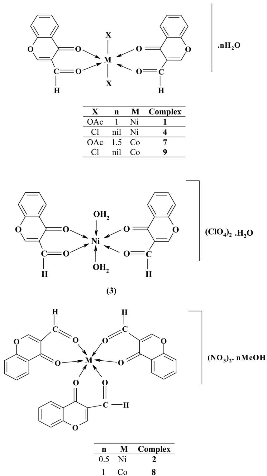
Scheme 2 Proposed structures of binary Ni(II) and Co(II) complexes.
