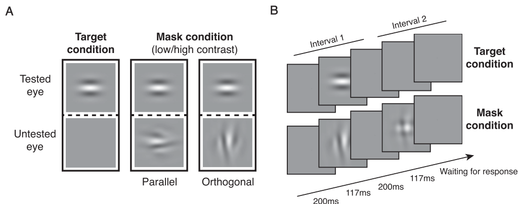
FIGURE 1. (A) Dichoptic stimuli. Target condition included one viewing condition: the 0^\circ Gabor target was presented to the tested eye and a mean luminance background was presented to the untested eye. Mask condition included 2 threshold mask conditions: (1) low contrast: the mask contrast was 3 times higher than the individual's contrast threshold; and (2) high contrast: the mask contrast was 10 times higher than the individual's contrast threshold. Each threshold mask condition included 2 orientation conditions: (1) parallel condition: the 0^\circ Gabor target was presented to the tested eye and the 0^\circ mask was presented to the untested eye; and (2) orthogonal condition: 0^\circ Gabor target was presented to the tested eye and the 90^\circ mask was presented to the untested eye. (B) Time course of the experiment. Each trial began with an orange fixation point (radius 0.1^\circ ) appearing for 200 ms. The first interval stimulus appeared for 117 ms without fixation point and signaled by a brief tone, followed by a 200 ms inter-stimulus interval with an orange fixation point. Then a 117 ms second stimulus interval appeared signaled by a brief tone, and a green fixation point until response. Response correctness was then indicated by another tone.
