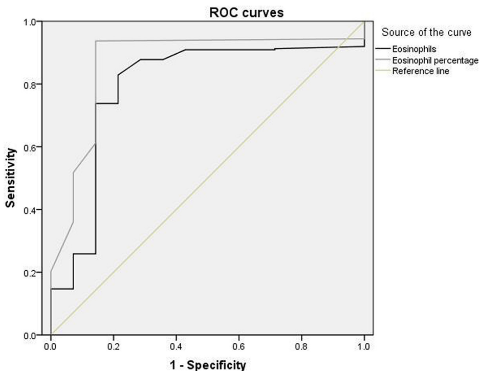
Figure 1: The receiver-operating characteristic(ROC) analysis for Eosinophils and Eosinophil percentage in predicting non-death.
