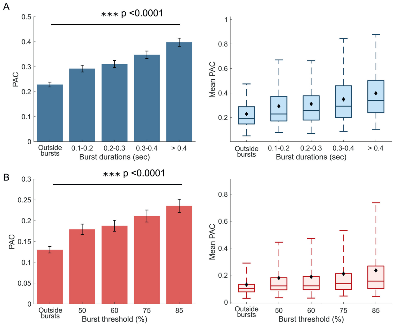
Fig. 9. PAC increases progressively with both burst duration and thresholds increments. A, Bar and box plots of PAC at different burst durations. PAC significantly increases with burst duration with longer bursts capturing higher levels of coupling. B, Bar and box plots of PAC at different burst thresholds. PAC increases significantly with threshold increments. All concentrated burst vectors were length adjusted.
