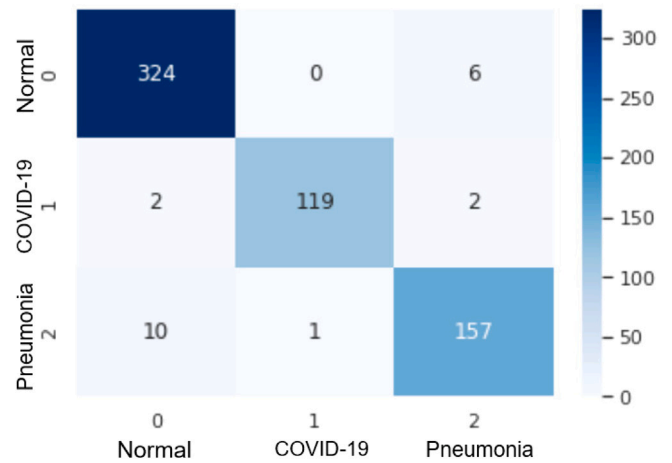
Fig. 9. Figure showcasing the Confusion Matrix of CoviXNet on 3-class classification.
