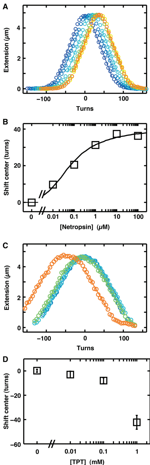
Figure 5. Effect of Netropsin and TPT on DNA rotation–extension behavior at low force. (A) Rotation–extension curves for a 20.6-kb DNA in the presence of increasing concentrations of netropsin, taken at F = 0.25 pN. Netropsin concentrations employed are (blue to red): 0, 0.01, 0.1, 1, 10 and 100 \mu\text{M} . Upon addition of netropsin, it is observed that rotation of the magnets by positive turns is required to recover the maximum of the rotation–extension curves. (B) Quantification of the number of positive turns required to recover the maximum of the
