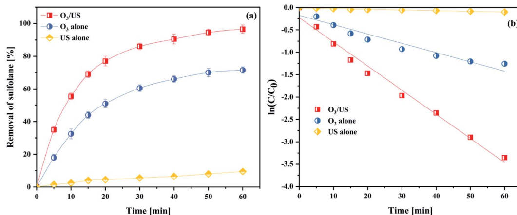
Fig. 11 (a) Comparison of different reaction systems in terms of the destruction of sulfolane; (b) kinetic data fitting for the sulfolane removal rate in different reaction systems (intake flow rate 300 L h -1 ; gaseous ozone concentration 32.38 mg L -1 ; US power 1000 W; temperature 293.15 K; initial sulfolane concentration 200 mg L -1 ).
