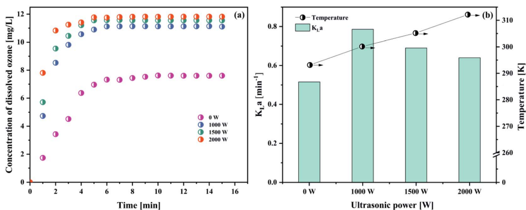
Fig. 8 (a) Variations in the dissolved ozone concentration with time under different ultrasonic powers, and (b) the corresponding K_L a value and system temperature (pH 3; intake flow rate 300 L h -1 ; gaseous ozone concentration 32.38 mg L -1 ; temperature 293.15 K).
