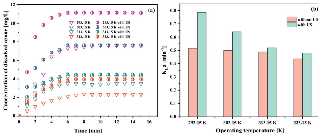
Fig. 7 Effect of operating temperature on (a) the concentration of dissolved ozone and (b) K_L a (pH 3; intake flow rate 300 L h -1 ; gaseous ozone concentration 32.38 mg L -1 ; US power 1000 W).
