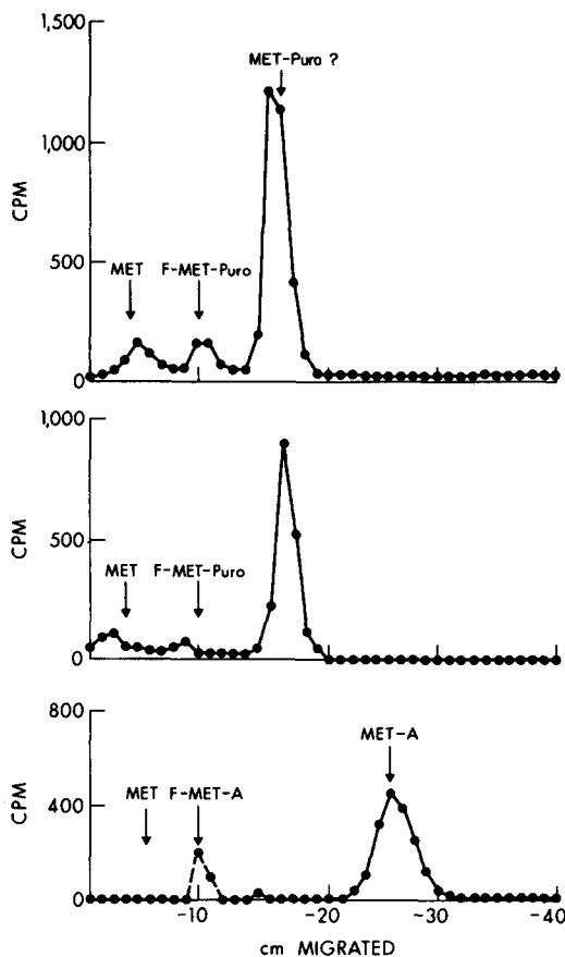
FIGURE 3 Product of mild acid hydrolysis of presumed f-Met-puromycin. 1.8 \times 10^8 cells were labeled with [ ^{14}\text{C} ]methionine (0.01 \mu\text{Ci}/\text{ml} ) for 2 min, treated with puromycin (0.15 mg/ml) for 14 min, homogenized, and acidified to pH 5.5. The homogenate was extracted with ethyl acetate, and the extract was subjected to high voltage electrophoresis in parallel with a sample of standard [ ^{14}\text{C} ]f-Met-puromycin. Material from the presumed f-Met-puromycin peak was eluted with methanol, the solvent distilled, made 0.2 N in HCl (Sheehan and Yang, 1958), sealed under a vacuum in glass ampules, and incubated at 37°C for 36 h. Samples were then neutralized and subjected to electrophoresis (70 min, 3,000 V) in pyridine-acetate buffer pH 3.5; chromatograms were cut into strips, eluted with \text{NH}_4\text{OH} , and radioactivity was determined in Bray's scintillant (Bray, 1960). Arrows within figures indicate mobilities of standard compounds. (Upper panel) HeLa cell extracts subjected to mild acid hydrolysis. (Middle panel) Standard [ ^{14}\text{C} ]f-Met-puromycin eluted and subjected to similar treatment. (Lower panel) Standards (Formyl-methionyl-adenosine) chromatographed in parallel and prepared as previously described (Galper and Darnell, 1969). These standards migrated as expected from structural and electro-
