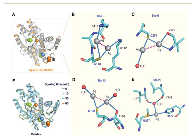
Fig. 3 Crystallographic analysis reveals the coordination geometries of the four silver-binding sites of MDH. (A) Overall structure of Ag-MDH-3. The coordination geometry of silver at the Cys113 site (B), Cys251 site (C), Cys109 site (D) and Met227/His177 site (E). \text{Ag}^+ ions are shown as grey spheres, water as red spheres, the argentophilic interactions in purple dash line and weak interactions between the O atom from Ile117/Val146 and \text{Ag}^+ ions shown as blue dash line. (F) Superimposition of Ag-MDH-1 (blue), Ag-MDH-2 (green), Ag-MDH-3 (yellow) with apo-MDH (grey) with RMSD of 0.233 \text{ \AA} , 0.312 \text{ \AA} , and 0.309 \text{ \AA} respectively. Structural alignment was done over C_\alpha residues using Dalilite.
