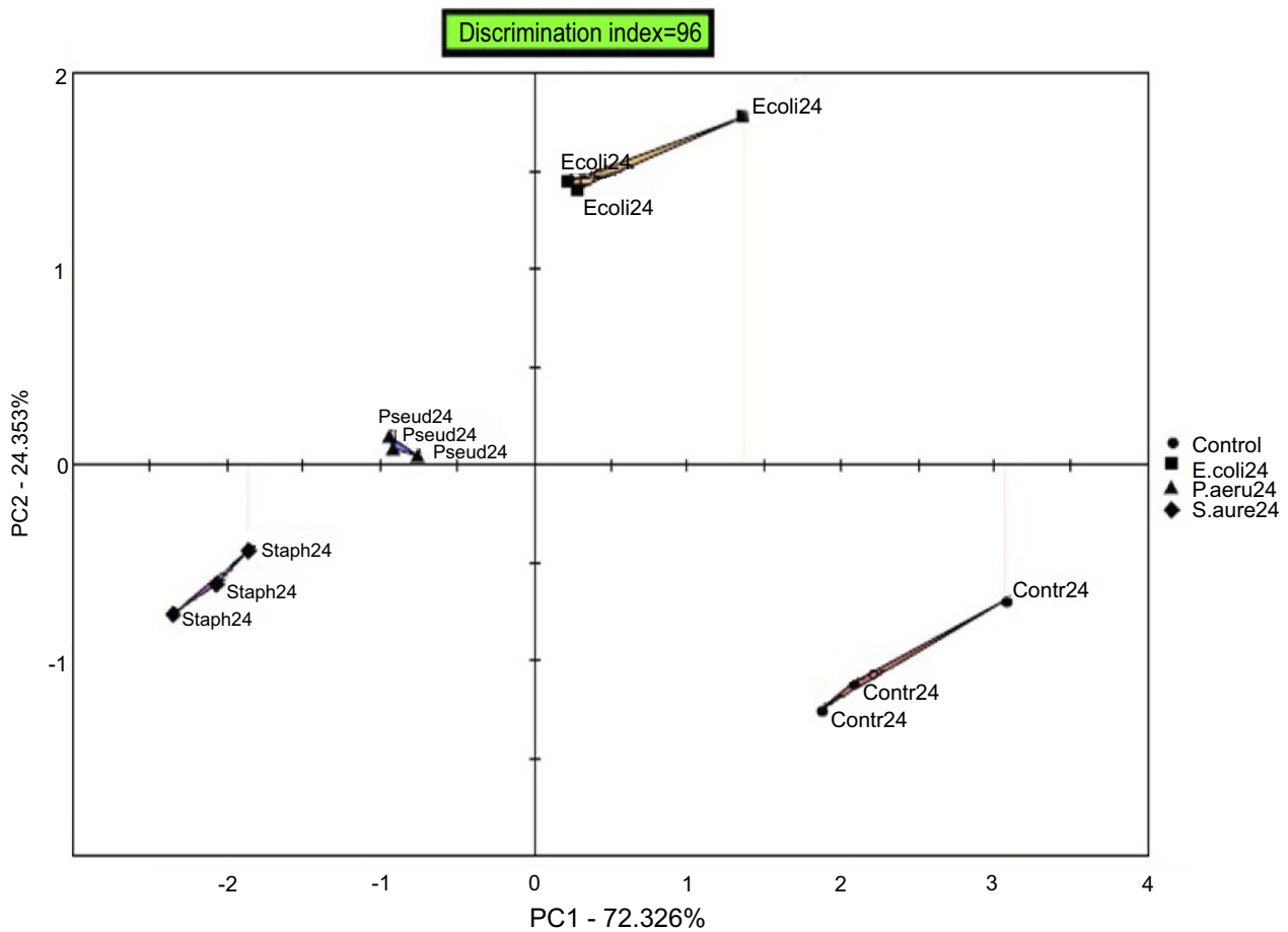
Figure 3 PCA scores plot of bacterial isolates ( Escherichia coli , Staphylococcus aureus , and Pseudomonas aeruginosa ) after 24 hrs of inoculation, showing high discrimination index value of 96 between samples. PC1 and PC2 explain 97% of the total variation. Abbreviation: PCA, Principal Component Analysis.
