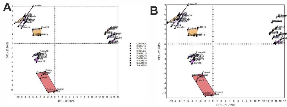
Figure 4 (A) DFA scores plot of bacterial isolates ( Escherichia coli , Staphylococcus aureus , and Pseudomonas aeruginosa ) after 15, 18, and 24 hrs of inoculation, (B) DFA model showing the projection and identification of unknown bacterial isolates near to E. coli . DF1 and DF2 explain 100% of the total variation.
