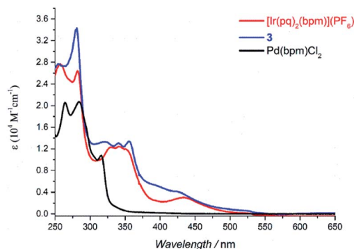
Fig. 2 UV-vis spectra of [Ir(pq) 2 (bpm)](PF 6 ), 3, and Pd(bpm)Cl 2 in DCM solution ( 5 \times 10^{-5} \text{ M} ).
