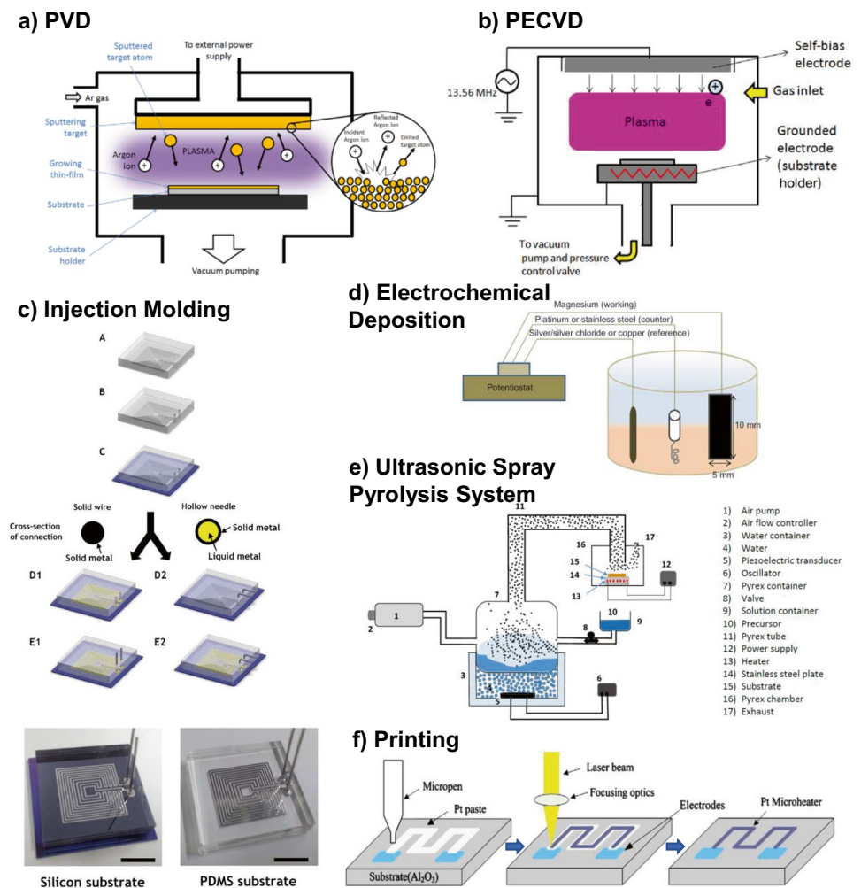
Fig. 11 Illustrations of the microheater fabrication process. (a) Schematic of PVD, (b) PECVD (Pessoa et al. 2015) Reprinted with permission from Elsevier, (c) Injection molding fabrication processes of liquid metal microheaters (Jinsol and Jungchul 2014) Reprinted with permission from IEEE, (d) Schematic of an electrochemical cell for the direct electrodeposition (Augello and Liu 2015) Reprinted with permission from Elsevier, (e) Illustrative of homemade spray pyrolysis system (Gharsi and Ansari 2016) Reprinted with permission from IOP, (f) Illustration of micro-pen direct writing and laser sintering fabrication procedure (Cai et al. 2011) Reprinted with permission from Elsevier
