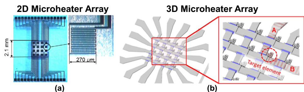
Fig. 9 (a) 2D 4 \times 4 microheater array with an enlarged view of heater (Jung et al. 2011) Retrieved with permission from Elsevier, (b) 3D microheater array with lead lines are grade crossings with overpasses (Horade et al. 2016) Retrieved with permission from CCSE
