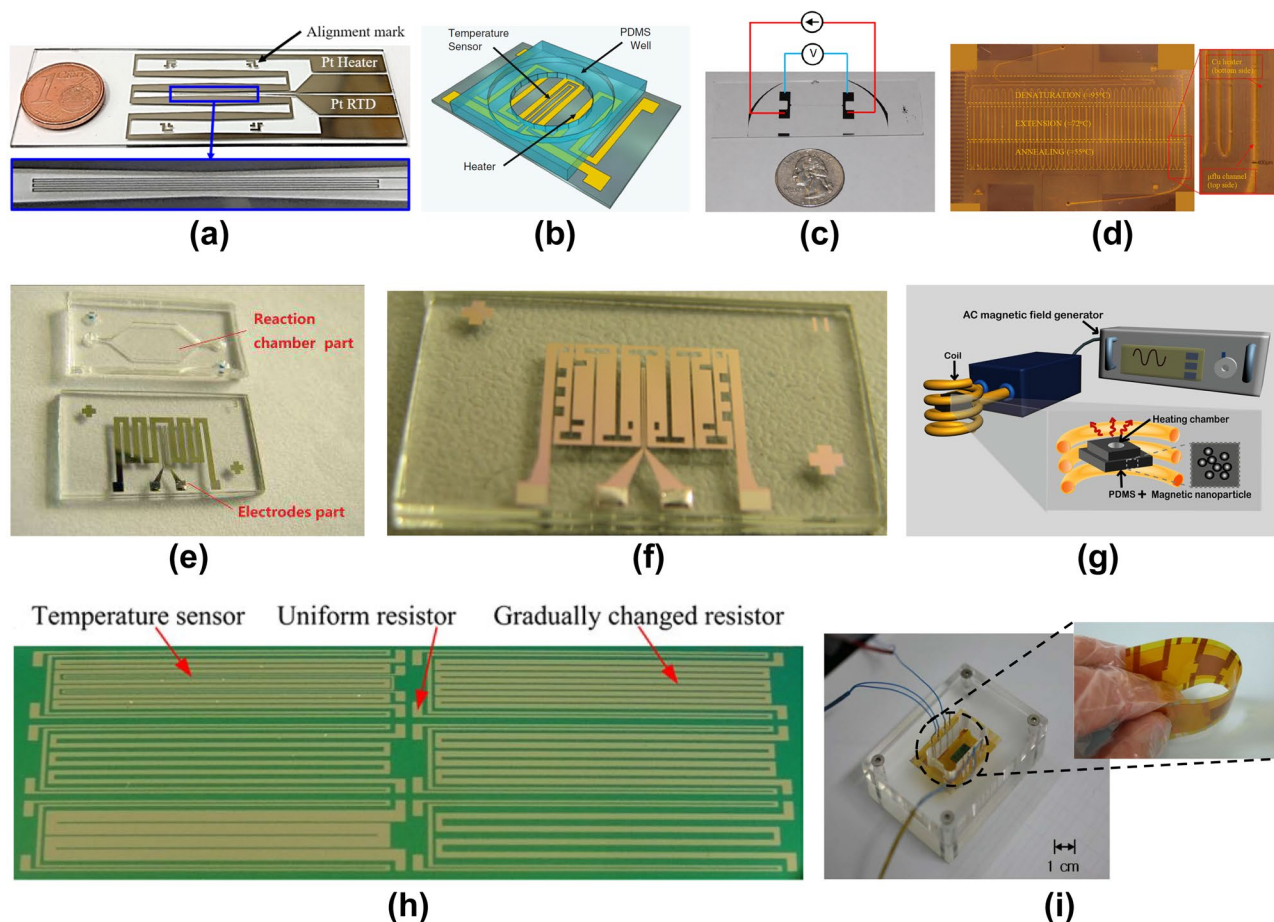
Fig. 20 Microheaters for DNA amplification. (a) Fabricated thin film heater/RTD PCR chip (Jeong et al. 2018), (b) Microheater and temperature sensor patterned glass slide (Hilton et al. 2012) Pictures reprinted with permission from Springer Nature, (c) External electrical circuit employed to drive the Ti microheater device (Javed et al. 2012) Reprinted with permission from AIP, (d) Photograph of a fabricated Cu heater in Cu-clad PI substrate (Moschou et al. 2014) Reprinted with permission from Elsevier, (e) PCR chip with reusable electrode part (Cao et al. 2015) Reprinted with permission from Trans Tech, (f)
