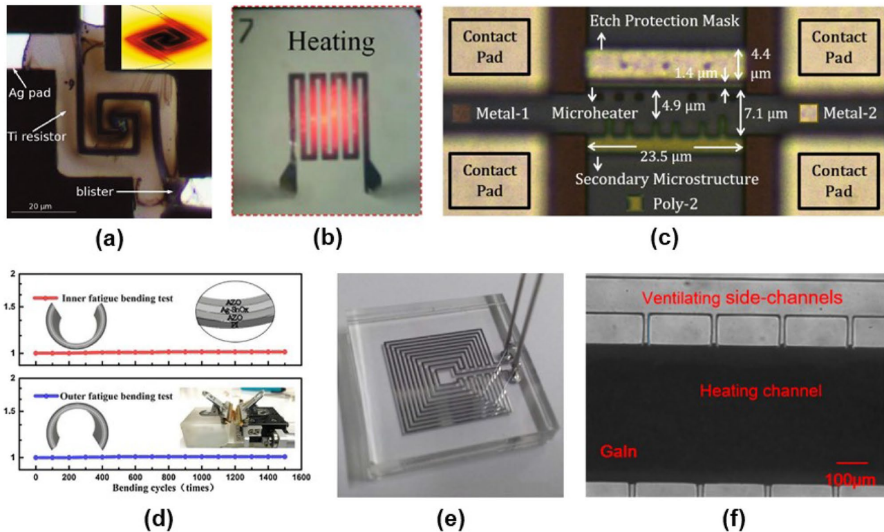
Fig. 4 Different microheater utilized by researchers (a) Ti/Ag microheater heating up to failure (Guan and Puers 2010) Reprinted with permission from Elsevier, (b) Cr–CrN, and CrN–Pt based microheater (Chang and Hsihe 2016) Reprinted with permission from Elsevier, (c) Optical micrograph of CNT growth structures in AMS 350 nm process (Roy et al. 2019) Reprinted with permission from
