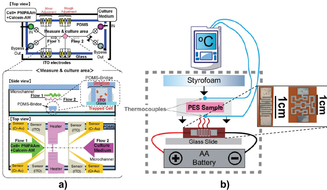
Fig. 19 Microheaters used in cell culturing and incubation. (a) Cell culturing temperature Controlled chip (Yamanishi et al. 2008) Reprinted with permission from IEEE, (b) Battery-powered incubation system with an enlarged view of two heater designs (Byers et al. 2019) Reprinted with permission from RSC
