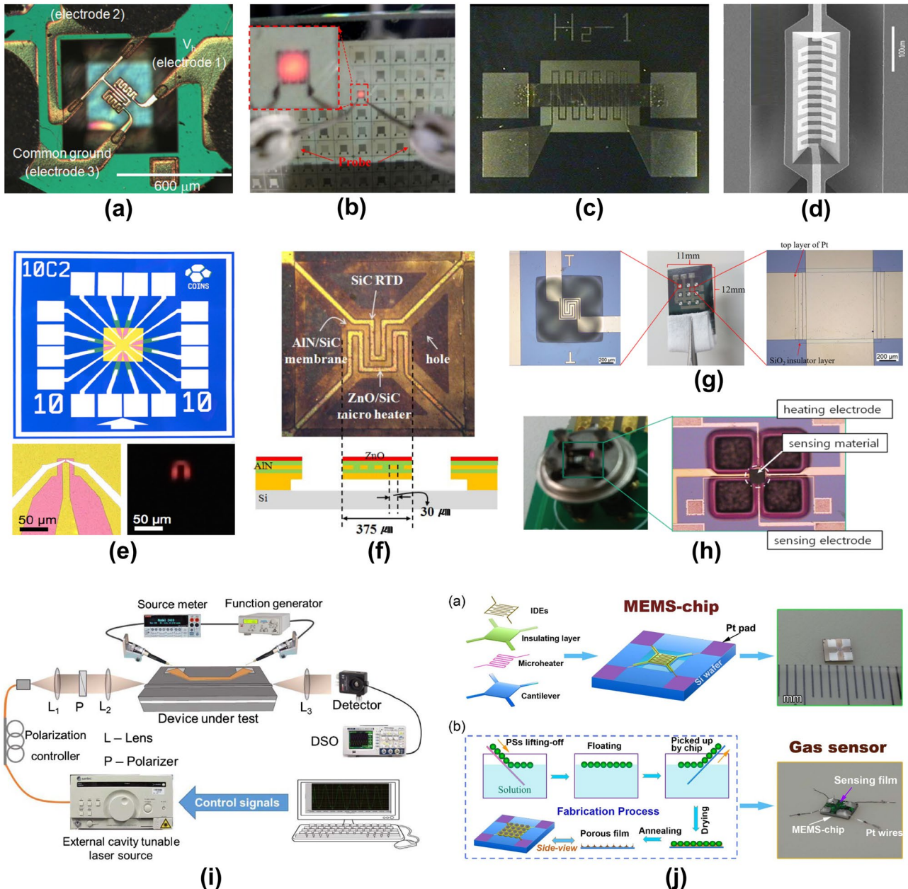
Fig. 17 Microheaters used in gas sensing. (a) optical image of the gas sensor with microheater and sensing electrode (Hwang et al. 2011a), (b) Micrographs of micro-hotplate on a glass substrate (Chang and Hsihe 2016), (c) Fabricated H 2 sensor (Yoon et al. 2012) Pictures retrieved with permission from Elsevier, (d) SEM image of the fabricated 3-D microheater (Xu et al. 2011) Retrieved with permission from IEEE, (e) Photograph of four SiC microheaters (Harley-Trochimczyk et al. 2017) Retrieved with permission from IOP, (f) NO gas sensor with integrated 3C-SiC microheater
