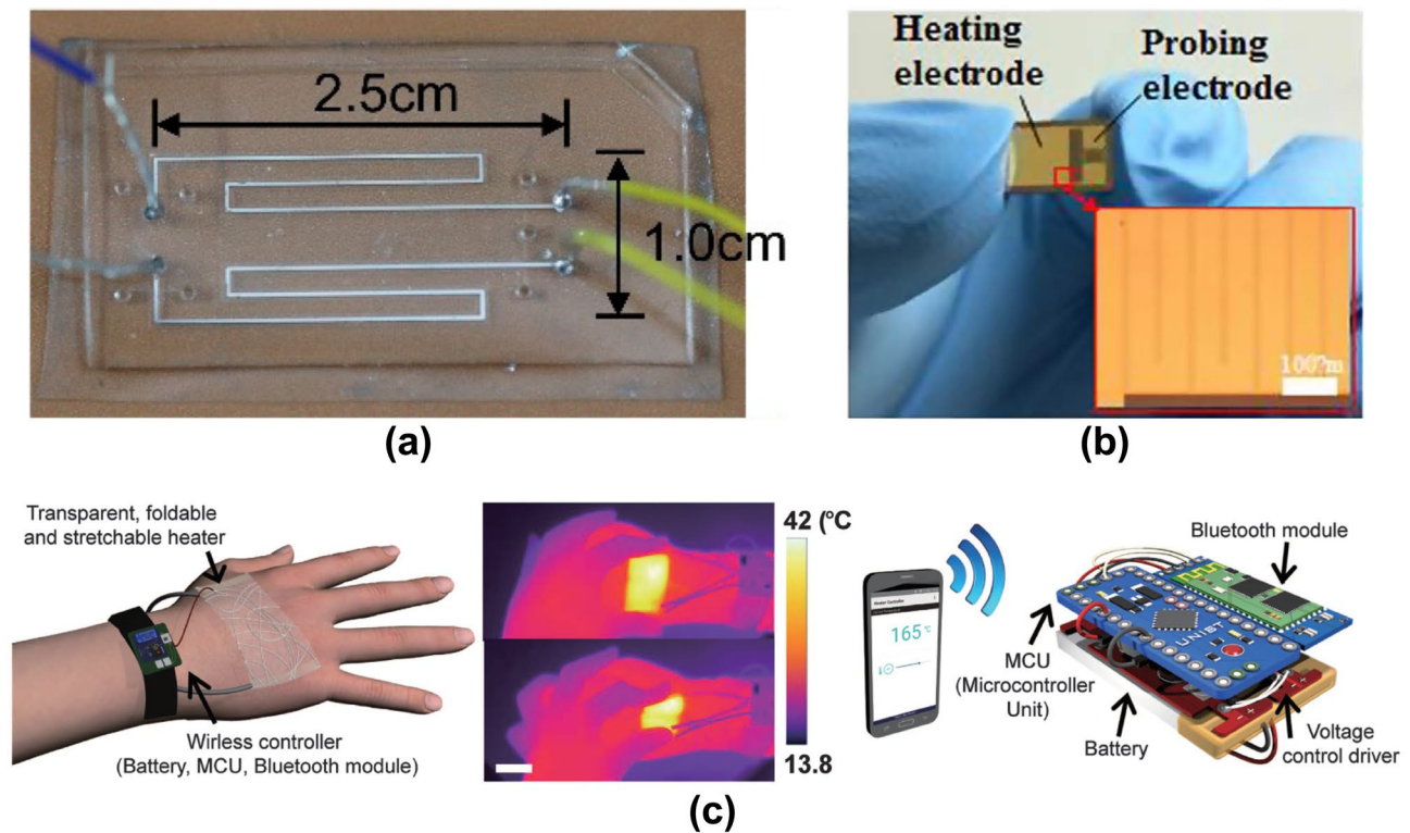
Fig. 22 (a) EGaIn liquid metal-based microheater (Zhang et al. 2020) Reprinted with permission from MDPI, (b) Temperature-controllable microheater chip for colour display devices (Kim et al. 2015), (c)
