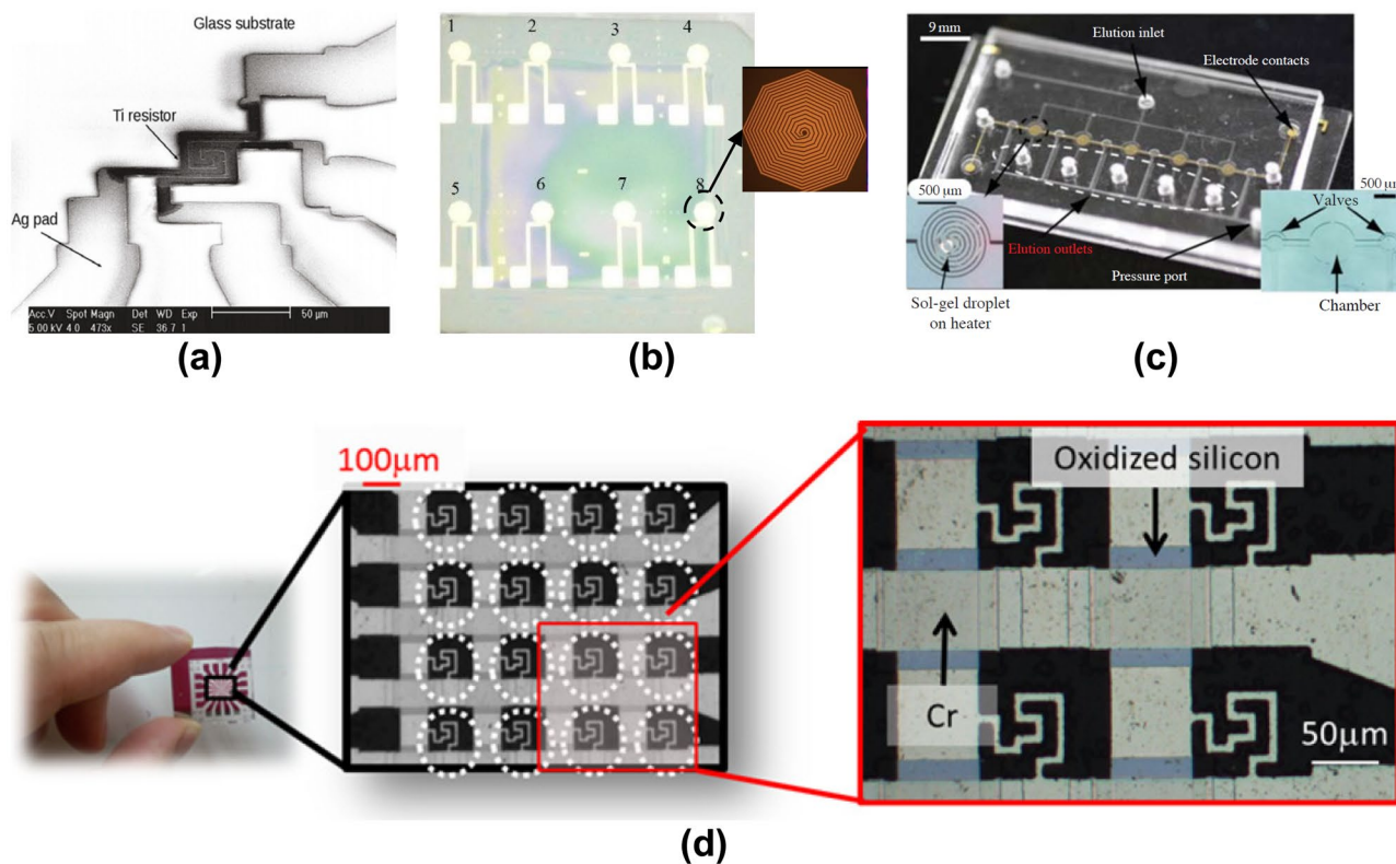
Fig. 21 Microheaters implemented in biochemical research. (a) SEM image of the Ag/Ti microheater (Guan and Puers 2010) Reprinted with permission from Elsevier, (b) Octogen gold heater on polyimide thin film substrate (Yu et al. 2015) Reprinted with permission from ASME, (c) Au/Cr microheater on the glass substrate for cross-
