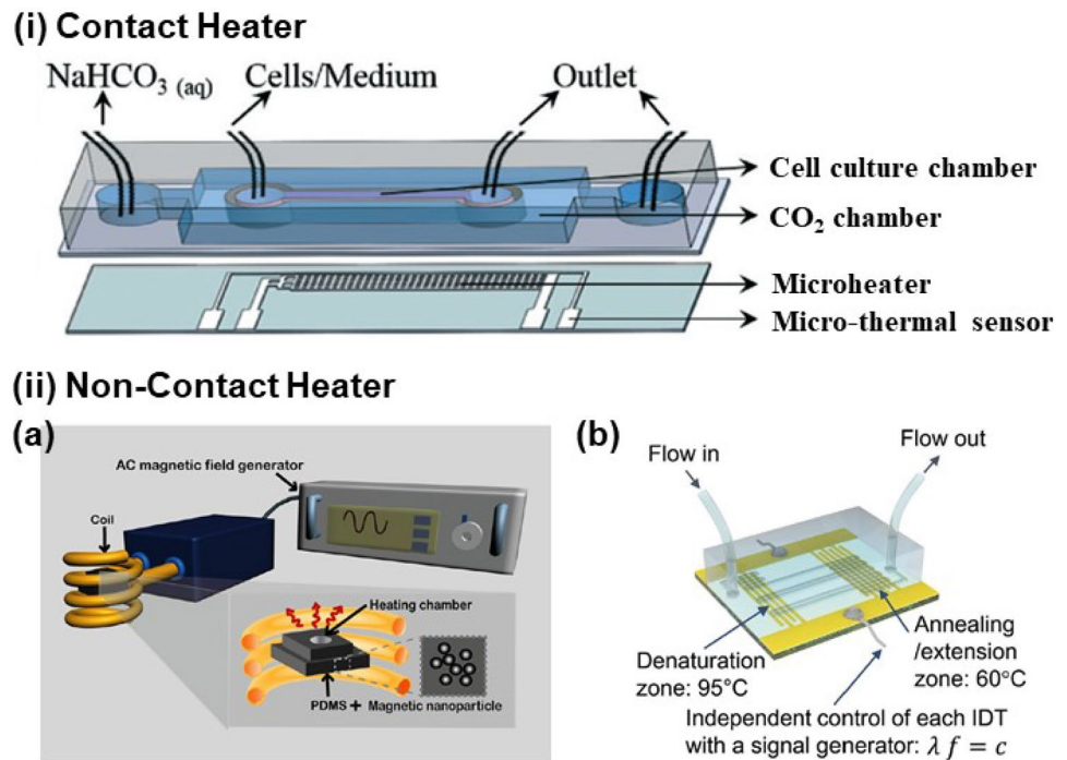
Fig. 2 External heating systems. (i) Contact heater (Yu et al. 2014) Reprinted with permission from RSC (ii) Non-contact heaters. (a) Schematic drawing of induction heating based on the magnetic nanoparticle-embedded PDMS (MNP-PDMS) chip (Kim et al. 2010) Reprinted with permission from IOP, (b) PDMS chip bonded on LiNbO 3 piezoelectric substrate (Ha et al. 2015) Reprinted with permission from Nature
