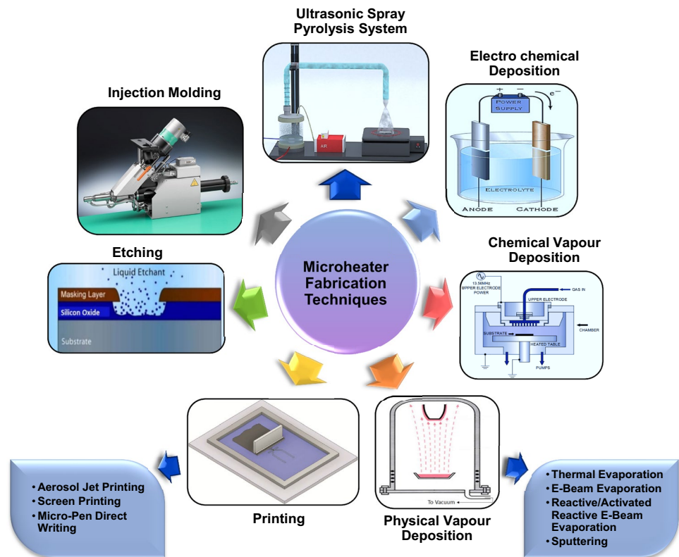
Fig. 10 Microheater fabrication techniques
