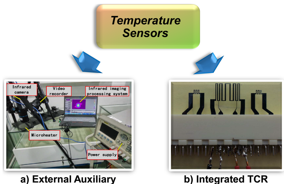
Fig. 13 Temperature sensors adapted in microheater temperature measurement (Li et al. 2017; Scorzoni et al. 2014) Retrieved with permission from Springer Nature and IEEE
