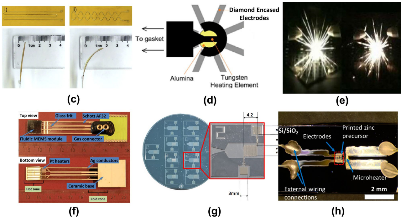
Fig. 23 (a) Microheater array for powder sintering (Holt et al. 2018) Reprinted with permission from Elsevier, (b) Curved CNT-film microheater array on PET for thermochromic displays (Liu et al. 2011) Reprinted with permission from Wiley, (c) Bending performance of actuators with different heater patterns at similar temperature (Cao and Dong 2019) Reprinted with permission from Elsevier, (d) Illustration of a Tungsten microheater designer anvil showing the eight diamond encased electrodes (Weir et al. 2009) Reprinted with permission from AIP, (e) Optic images of combustion flame in the
