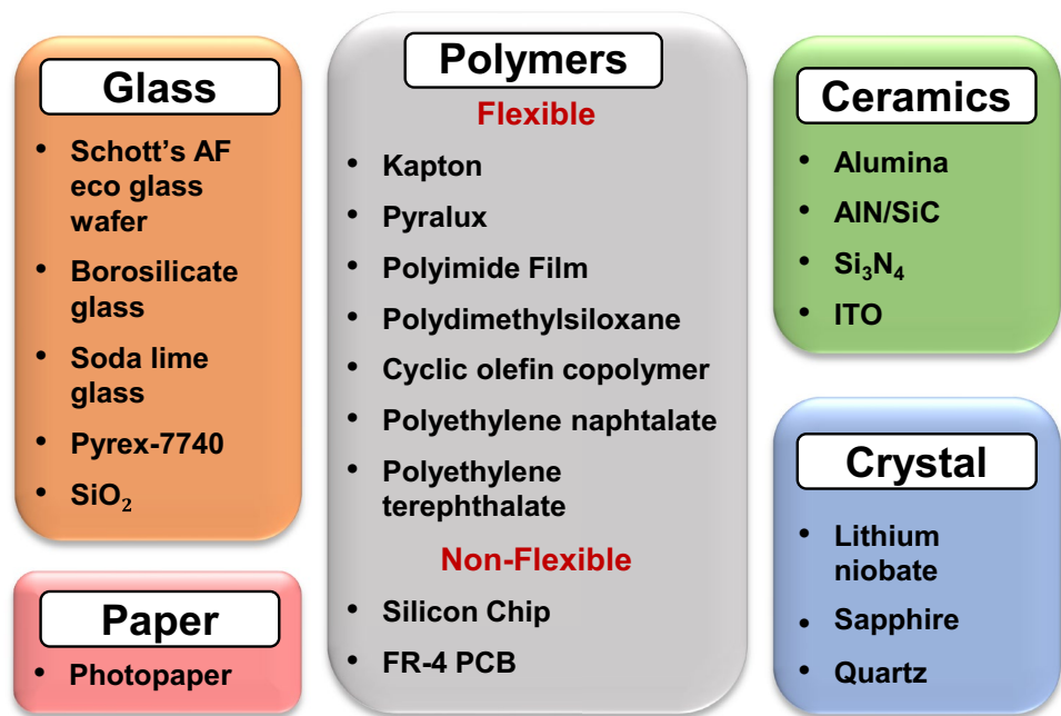
Fig. 5 Classification of the various substrate for microheater so far investigated by various researchers
