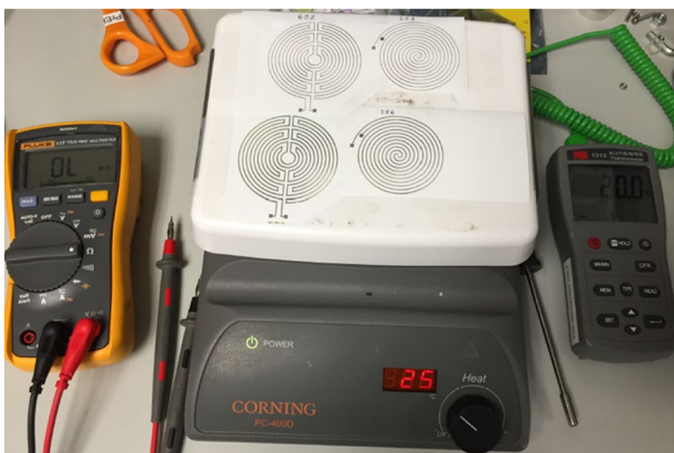
Fig. 14 Setup to determine TCR of the nano-silver ink microheater (du Plessis et al. 2017) Retrieved with permission from SPIE
