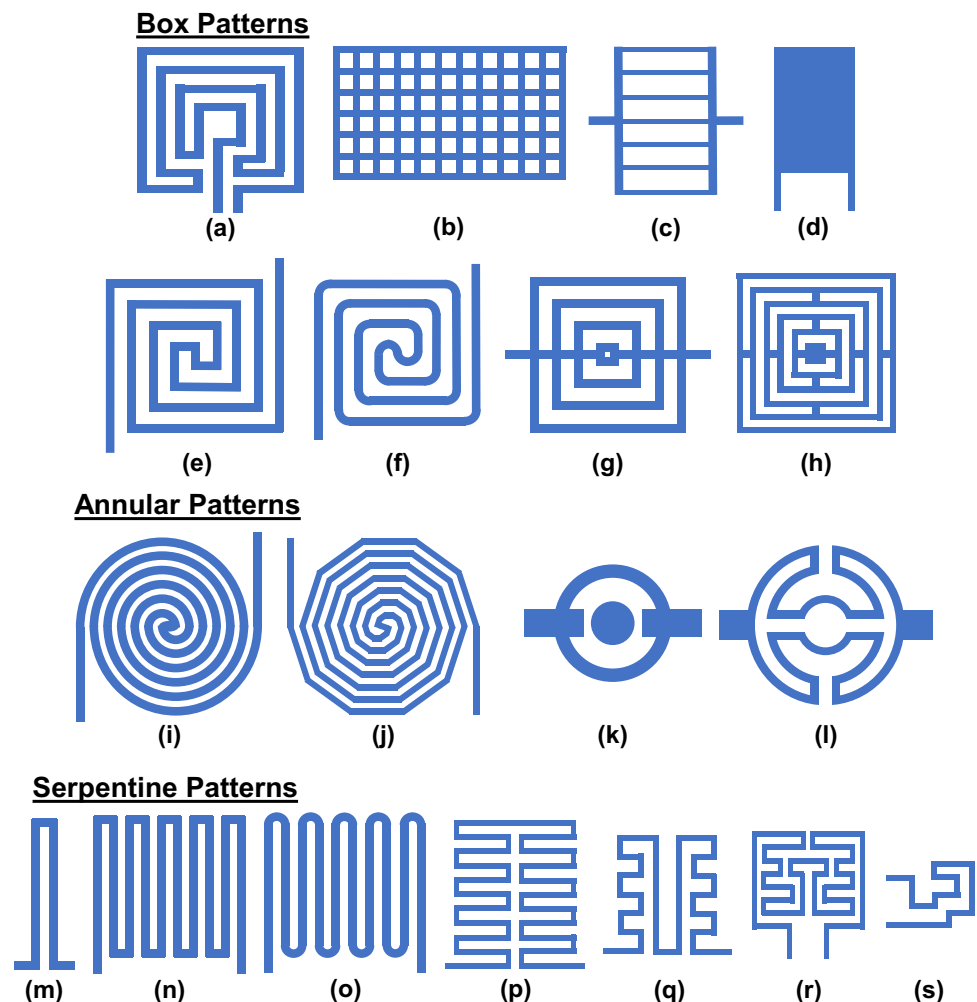
Fig. 8 Illustrative diagram of different microheater designs so far investigated by various researchers (Botau et al. 2015; Das and Kakoty 2015; Ha et al. 2015; Han and Meyyappan 2016; Hasan et al. 2016; Holt et al. 2017; Horade et al. 2016; Hwang et al. 2011a; Jinsol and Jungchul 2014; Kim et al. 2010; Lee et al. 2013; Nieto et al. 2017; Petrucci et al. 2015; Rajput et al. 2018; Roy et al. 2010; Ruiqi et al. 2011; Wu et al. 2009; Yu et al. 2017; Zhong et al. 2009). (a) Inverted C shaped, (b) Rectangular mesh pattern, (c) Lines, (d) Plate, (e) Double spiral Square, (f) Curved double spiral square, (g) Ring-shaped, (h) Square gridded, (i) Double spiral, (j) Octogen, (k) Circular, (l) Dual C, (m) Inverted U, (n) Meander, (o) Meander with rounded corners, (p) Dual meander, (q) U Dual meander, (r) Wing, (s) Hook
