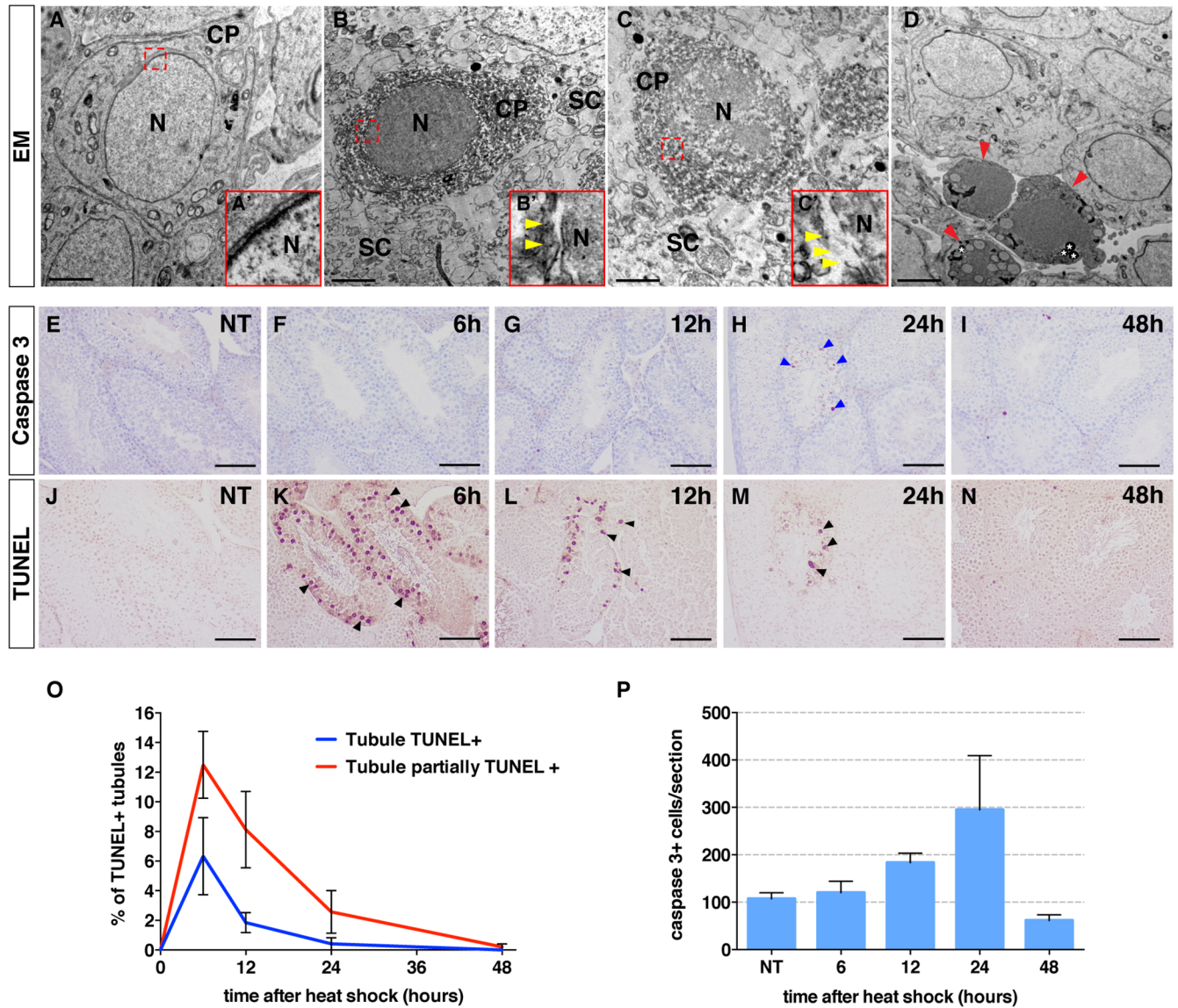
Fig 5. Mild hyperthermia induces germ cell necrosis during mouse spermatogenesis. (A–D) Electron micrographs of non-treated (A) or heat-shocked mice testes at 6 (B–C) and 24 hours (D) after heat shock, showing cellular morphological hallmarks of necrosis (B–C) or apoptosis (D, red arrowheads). White asterisks indicate extranuclear densities observed in the cytoplasm that may reflect an unrelated acid phosphatase activity previously observed in GCs (D [67]). Insets (red squares in A–C) show ruptured nuclear membranes (yellow arrowheads in B' and C'). N and CP indicate nucleus and cytoplasm, respectively. SC indicates Sertoli cells. (E–I) Sections of non-treated (NT, E) or heat-shocked testes from 6–8-week-old wild-type mice stained with anti-cleaved caspase-3 antibody (E–I) at the indicated time after heat-shock. Blue arrowheads (H) indicate cleaved caspase-3 + cells. Scale bar, 100 μm. (J–N) Sections of non-treated (NT, J) or heat-shocked testes from 6–8-week-old wild-type mice stained with TUNEL (J–N) at the indicated time after heat-shock. Black arrowheads (K–M) indicate TUNEL + cells. Scale bar, 100 μm (J–N). (O) Quantification of the total fraction of tubules containing TUNEL + cells (blue curve) and the fraction of tubules partially filled with TUNEL + cells (red curve) at the indicated time after heat shock. (P) Quantification of activated caspase-3 + cells per section (mean ± s.e.m) at the indicated times after heat shock.
