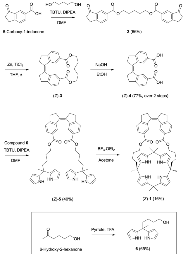
Scheme 2 Synthesis of stiff-stilbene strapped calix[4]pyrrole receptor ( Z )- 1 .
