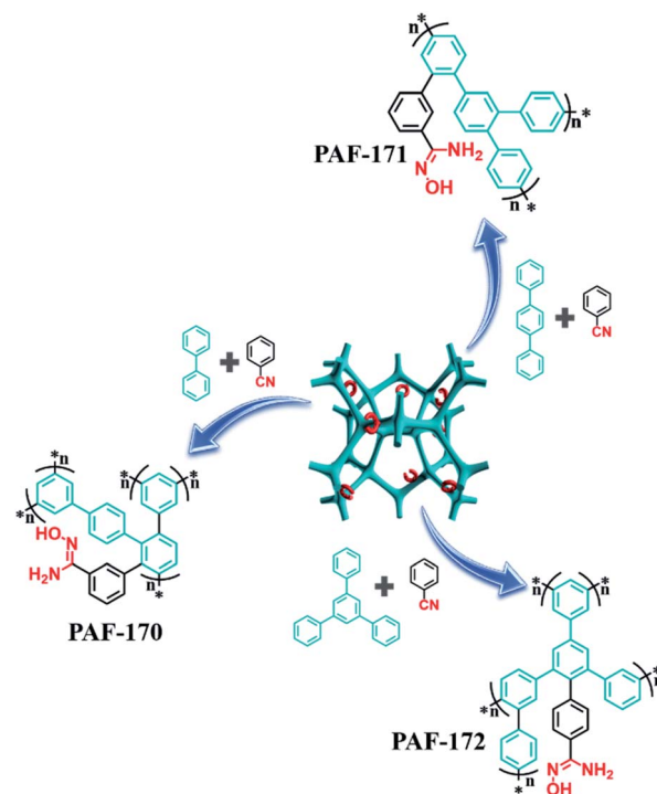
Fig. 1 Scheme of synthesis for PAF-AOs: \text{AlCl}_3/\text{CHCl}_3 , 60\text{ }^\circ\text{C} , 48\text{ h} . \text{NH}_2\text{OH}\cdot\text{HCl}/\text{Ni}(\text{CH}_2\text{CH}_3)_3/\text{EtOH} , 70\text{ }^\circ\text{C} , 48\text{ h} .
