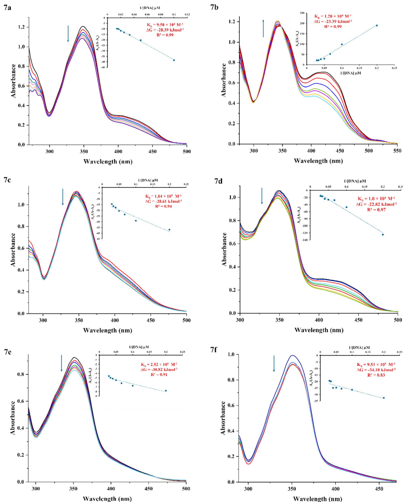
Fig. 1 UV-vis absorption spectra of compounds ( 7a–f ) at pH 7.4 and room temperature, with and without varying SS-DNA concentrations (5–35 μM), demonstrating spectral shifts indicative of groove binding interactions. Inset: plot of A_0/(A - A_0) as a function of 1/[DNA] .
