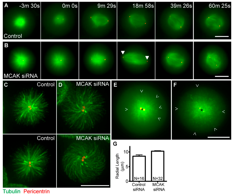
Figure 1. MCAK depletion results in transient long spindles after monastrol washout. (A) A cell treated with control siRNA. (B) A cell treated with MCAK-specific siRNA (arrowheads highlight centrosome position in long spindle). (C and D) Cells treated with control siRNA (C) or MCAK-specific siRNA (D) labeled with antitubulin and antipericentrin. Microtubule length can be measured in live cells expressing GFP-EB3 (green) and RFP-pericentrin (red). (E and F) The longest visible microtubule ends were measured in control (E) or MCAK siRNA-depleted (F) cells from the EB3-labeled tips (open arrowheads) to the center of the centrosomes (black asterisks). (G) Cell means of microtubule length in monasters in control siRNA and MCAK siRNA-depleted live cells. MCAK-depleted cells possess microtubules that are significantly longer ( P < 0.001 ). Error bars correspond to SEM of cell means of the longest measurable microtubules. Bars, 10 \mu\text{m} .
