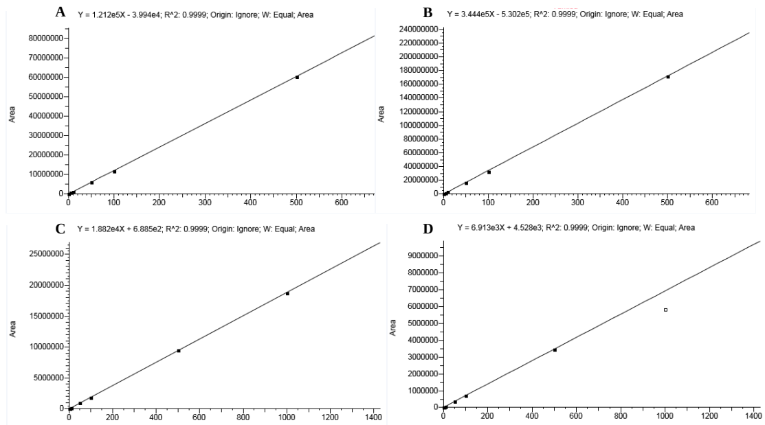
Fig. S1 Calibration curves for IAA, ZR, GA 3 and ABA standards obtained from HPLC-MS/MS analysis. a: IAA; b: ZR; c: GA 3 ; d: ABA.
