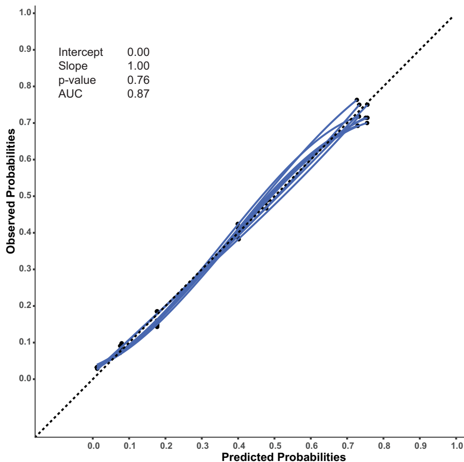
FIGURE 1 Calibration plot showing the performance of the MACS score chart in the 10 imputed datasets. AUC, area under the curve of the MACS score chart; Intercept, pooled calibration intercept; p-value, p-value of the Hosmer-Lemeshow test; slope, pooled calibration slope
