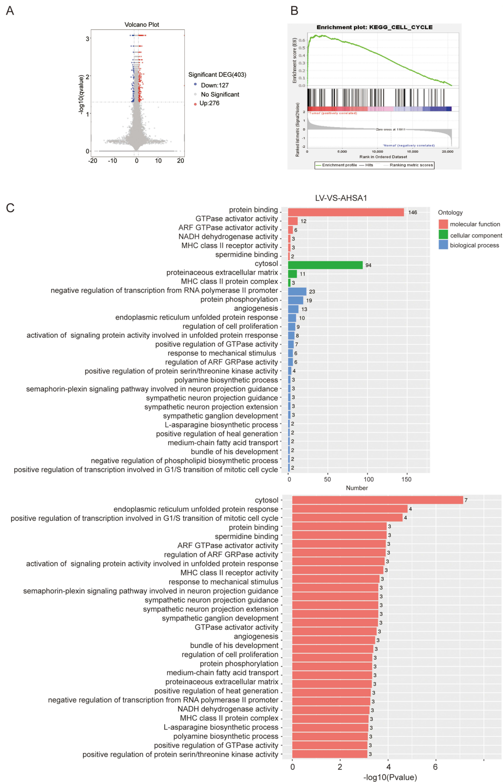
Figure 3 AHSAI-related signaling pathways analysis based on RNA-seq. (A) DEGs between the low- and high- AHSAI expression subgroups. (B) GSEA analysis was used to evaluate the abundance of main signaling pathways. (C) GO functional enrichment analysis of the molecules interacting with AHSAI.
