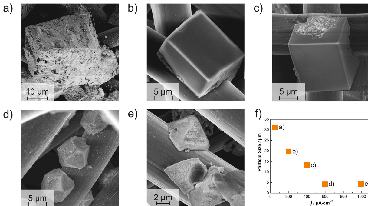
Figure 2. Scanning electron microscopy images from ex situ analysis of cathodes of fully discharged batteries, showing the discharge product NaO 2 : (a) 50 \mu\text{A}\cdot\text{cm}^{-2} ; (b) 200 \mu\text{A}\cdot\text{cm}^{-2} ; (c) 400 \mu\text{A}\cdot\text{cm}^{-2} ; (d) 600 \mu\text{A}\cdot\text{cm}^{-2} ; (e) 1,000 \mu\text{A}\cdot\text{cm}^{-2} ; (f) Particle size (maximal edge length) measured in the image as a function of discharge current density j .
