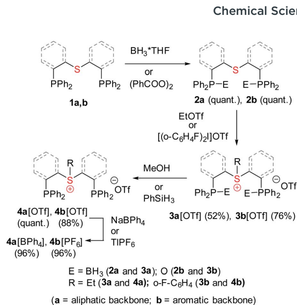
Scheme 1 Synthesis of aliphatic and aromatic sulfonium pincer ligands.
