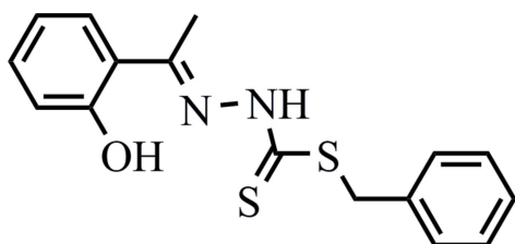
Figure 1 Chemical scheme of S -benzyl- \beta - N -(2-hydroxyphenylethylidene)dithiocarbazate (systematic name: benzyl 2-[1-(2-hydroxyphenyl)ethylidene]-hydrazinecarbodiithioate).
