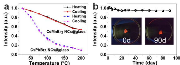
Fig. 5 The stability of \text{CsMnBr}_3 NC embedded glasses. (a) Relative intensity for the \text{CsMnBr}_3 NCs@glass and \text{CsPbBr}_3 NCs@glass sample in the temperature range of 25\text{--}200^\circ\text{C} . (b) Relative intensity for the \text{CsMnBr}_3 NCs@glass sample after soaking in water for different times. Inset shows photographs of \text{CsMnBr}_3 NC embedded glasses soaking in water under UV light for 0 and 90 days.
