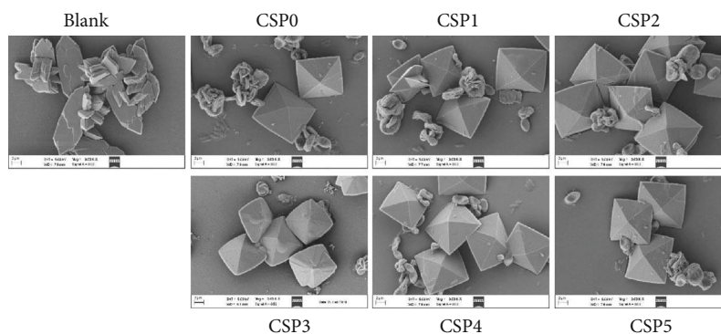
FIGURE 5: SEM images of CaOx crystals formed in the presence of 0.5 mg/mL CSPi. c(\text{Ca}^{2+}) = c(\text{Ox}^{2-}) = 0.60 mmol/L, c(\text{NaCl}) = 10 mmol/L; crystal growth time: 3 d. Magnification: 3000x.
