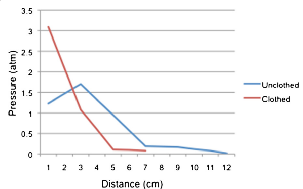
Figure 5 Pressure exerted on the bone by the bullet passage at varying distances from the bone. The clothed and unclashed samples are compared.
