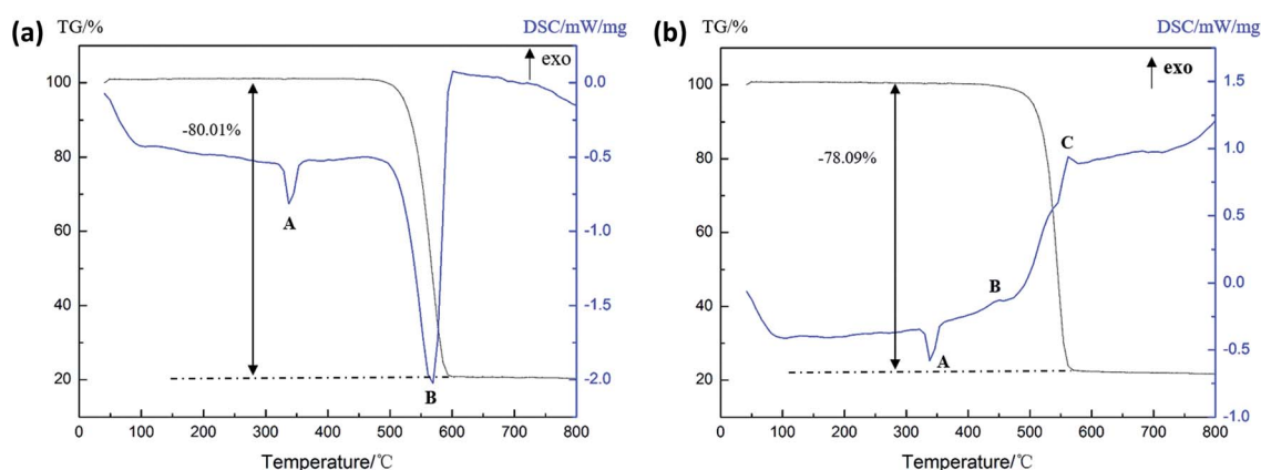
Fig. 9 The TG-DSC curves of (a) \text{Al}_2\text{O}_3 (1 \mu\text{m} )/PTFE and (b) \text{Al}_2\text{O}_3 (30 nm)/PTFE.
