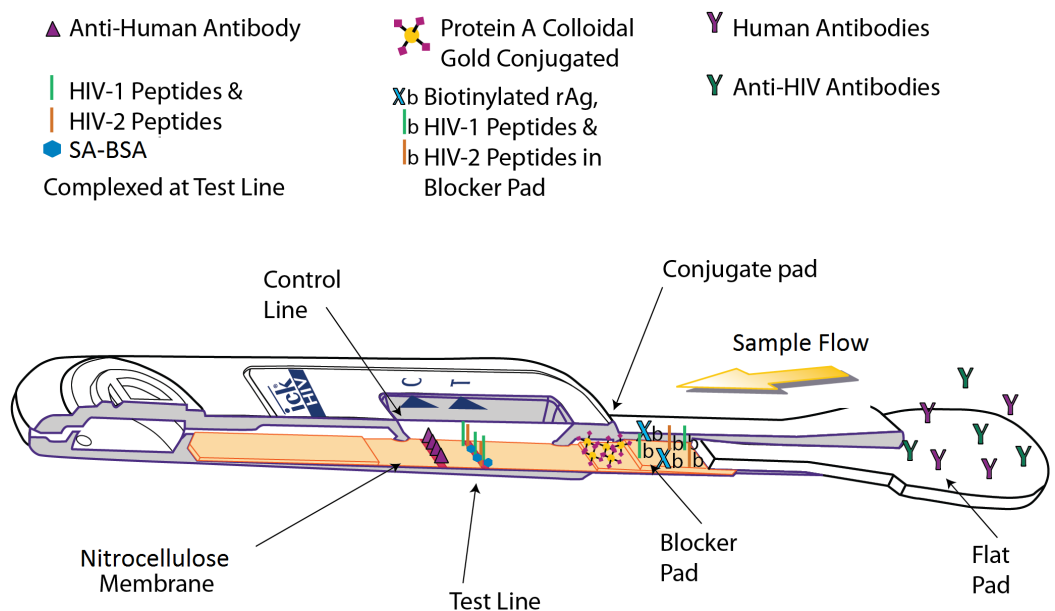
Figure 3 Operating principle of the OraQuick ADVANCE® Test. Sample is wicked up the device, hydrating blocker and conjugate pad reagents, which are transferred to the nitrocellulose membrane. HIV antibodies in the sample bind biotinylated reagents and are labeled by Protein A colloidal gold. The immuno-sandwich is immobilized by biotin binding with Streptavidin-BSA, and by anti-HIV antibodies interacting with anchored peptides at the test line. Human antibodies complexed with Protein A colloidal gold are captured at the control line. Accumulation of colloidal gold at the control and test lines creates a reddish-purple stripe.
