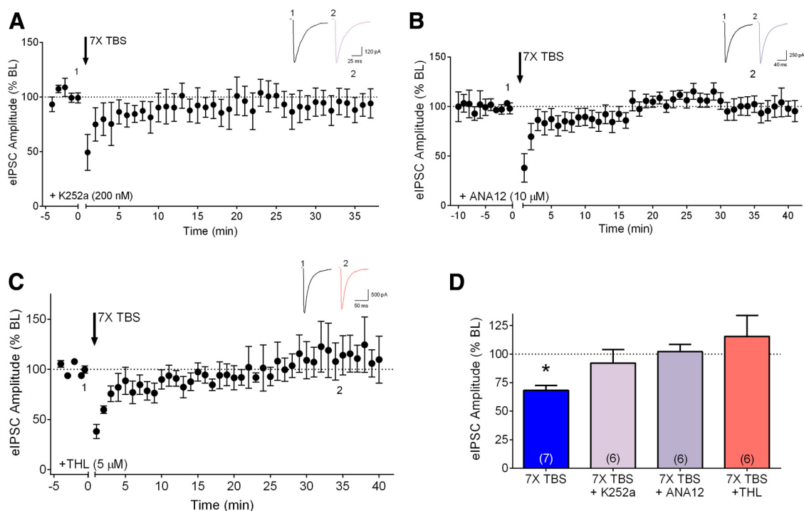
Figure 3 eCB-mediated iLTD requires endogenous BDNF signaling as well as DGL. A , Group time course showing the lack of effect of seven trains of TBS (7× TBS) on peak eIPSC amplitude in the presence of the tyrosine kinase inhibitor K252a (200 nM, n = 6 ). B , Group time course showing the lack of iLTD in response to 7× TBS in the presence of the trkB receptor antagonist ANA12 (10 \mu M, n = 6 ). Inset, Averaged sample sweeps during baseline (1) and 35 min after TBS (2) from a representative experiment. C , Group time course showing the lack of iLTD in response to 7× TBS in the presence of DGL inhibitor THL (5 \mu M, n = 6 ). D , Compiled group data for normalized eIPSC amplitude at 35 min postinduction in the presence of K252a (light pink bar), ANA-12 (light purple bar), or THL (coral bar). The effect of 7× TBS in vehicle (blue bar) was taken from Figure 2C for comparison. * p < 0.05 compared to baseline.
