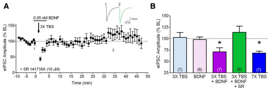
Figure 5 Synergized iLTD requires CB1R signaling. A , Group time course illustrating the lack of effect of 3× TBS-5 min BDNF combination on eIPSC amplitude in the presence of CB1R antagonist SR 141716A (SR, 10 \mu M, n = 6 ). Inset, Averaged sample sweeps during baseline (1) and 35 min after TBS (2) from a representative experiment. B , Compiled group data for normalized eIPSC amplitude at 35 min post various induction conditions. Hatched light blue bar, 3× TBS. Hatched pink bar, 0.05 nM BDNF for 5 min. Purple bar, Combination of 5 min-0.05 nM BDNF and 3× TBS. Green bar, Combination of 5 min-0.05 nM BDNF and 3× TBS, in the presence of SR. Blue bar, 7tr-TBS (taken from Fig. 2C for comparison).
