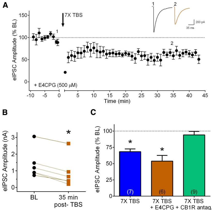
Figure 2 iLTD at layer 2/3 inhibitory synapses is independent of mGluR signaling. A , Group time course of the effect of 7× TBS on peak eIPSC amplitude in the presence of the group I/II mGluR antagonist E4CPG (500 μM; n = 6). Inset, Averaged sample sweeps during baseline (1) and 35 min after TBS (2) from a representative experiment. B , Data from individual experiments showing eIPSC amplitude baseline (black circles, BL) and 35 min after TBS in the presence of E4CPG (orange squares). * p < 0.05 compared to baseline. C , Compiled group data for normalized eIPSC amplitude 35 min after 7× TBS in vehicle (blue bar), E4CPG (orange bar), or CB1R antagonists (CB1R antagon., green bar). Numbers on bars indicate number of cells in each group (this and all following figures).
