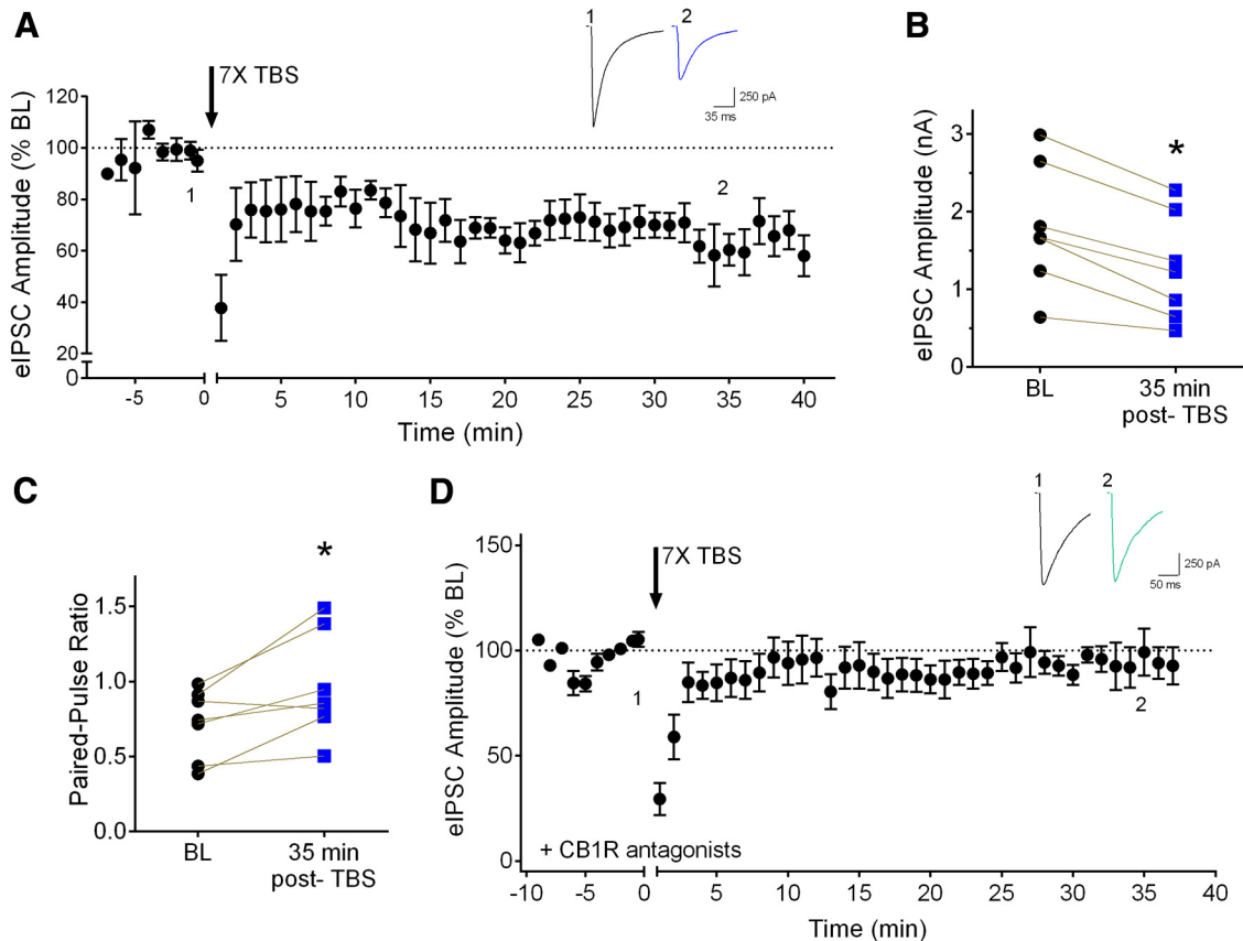
Figure 1 TBS in layer 2/3 induces CB1R-dependent iLTD. A , Group time course of the effect of seven trains of TBS ( 7\times TBS) on normalized peak eIPSC amplitudes ( n = 7 ). Arrow indicates TBS stimulation (this and all following figures). Inset, Averaged sample sweeps during baseline (1) and 35 min after TBS (2) from a representative experiment. B , Data from individual experiments showing eIPSC amplitude during baseline (black circles, BL) and 35 min after TBS (blue squares). *p < 0.05 compared to baseline. C , Paired-pulse ratio data from the same cells as in B during baseline (black circles, BL) and 35 min after TBS (blue squares). *p < 0.05 compared to baseline. D , Group time course showing lack of effect of 7\times TBS on peak eIPSC amplitude in the presence of the CB1R antagonists AM251 ( 5 \mu\text{M} ) or SR 141716A ( 10 \mu\text{M} , n = 9 in total). Inset, Averaged sample sweeps during baseline (1) and 35 min after TBS (2) from a representative experiment.
