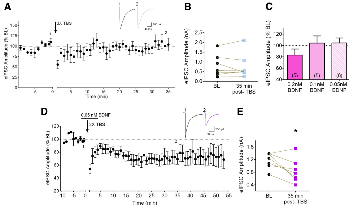
Figure 4 Low concentration of BDNF synergizes with subthreshold TBS to induce iLTD. A , Group time course of the effect of three trains of TBS (3× TBS) on normalized peak eIPSC amplitude. Inset, Averaged sample sweeps during baseline (1) and 35 min after TBS (2) from a representative experiment ( n = 7 ). B , Data from individual experiments showing eIPSC amplitude baseline (black circles, BL) and 35 min after 3× TBS (light blue squares). C , Dose response of the acute effect of BDNF (5 min) on eIPSC amplitude. Left bar, 5 ng/ml (0.2 nM) BDNF; middle bar, 2.5 ng/ml (0.1 nM) BDNF; right bar, 1.25 ng/ml (0.05 nM) BDNF. D , Group time course of peak eIPSC amplitude under the combination of 3× TBS and 5 min-0.05 nM BDNF. Horizontal bar above trace indicates BDNF application. E , Data from individual experiments showing eIPSC amplitude during baseline (black circles, BL) and 35 min after 3× TBS and 5 min-0.05 nM BDNF (purple squares). Time window is relative to TBS (for this and Fig. 5). * p < 0.05 compared to baseline.
