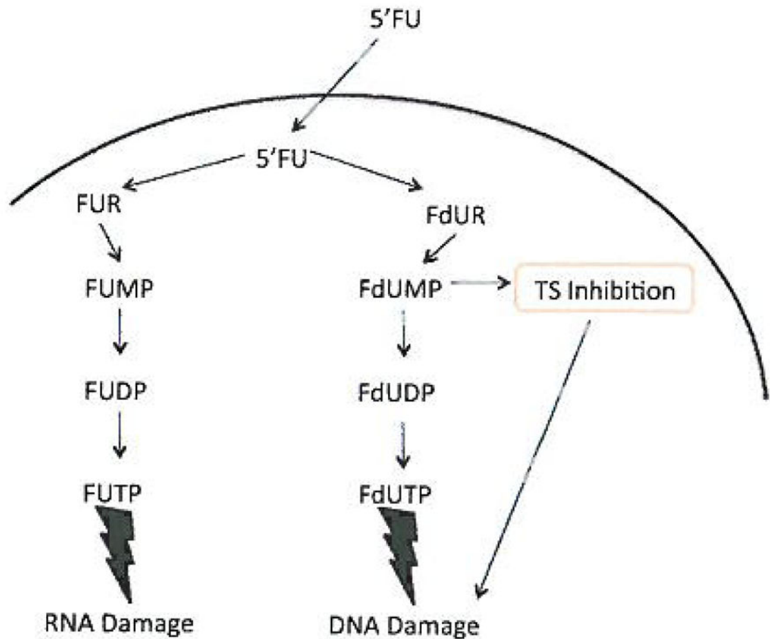
Figure 2. Mechanism of 5FU leading to RNA and DNA damage. Thymidylate synthase inhibition is the main mechanism of action of 5FU through its active metabolite FdUMP. Synthesis of the pyrimidine thymidine, which is required for DNA synthesis, is the result of blocking thymidylate synthase. Thymidylate synthase methylates deoxyuridine monophosphate (dUMP) to form thymidine monophosphate (dTMP). The use of 5FU in cancer causes there to be a reduction leading to a scarcity of dTMP so that rapidly dividing cancer cells die from a lack of thymine.
