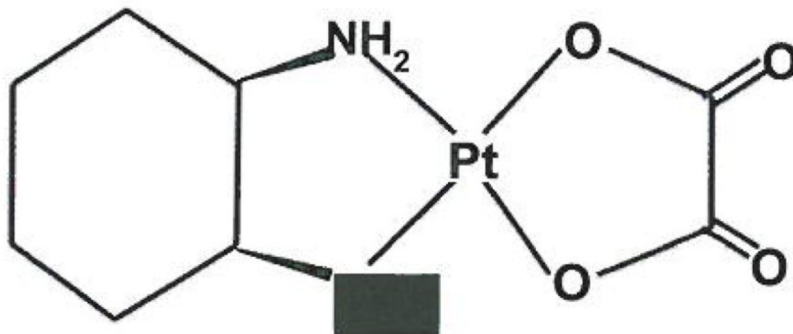
Figure 6. Similar to Cisplatin, Oxaliplatin contains a doubly charged platinum ion in the center. It, however, contains diamnocylohexane and carboxylate compounds. These platinum complexes bind to and crosslink DNA in vivo which triggers apoptosis.
