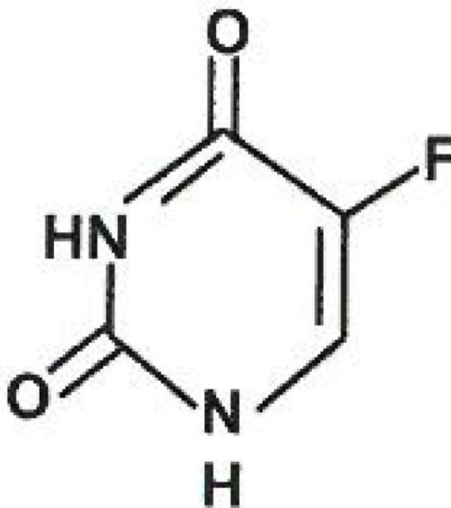
Figure 1. Structure of 5FU with the fluor group in carbon 5-position. 5FU is a pyrimidine analog drug whose mechanism of action is through irreversible inhibition of thymidylate synthase (TS). Clinically is have been used in the treatment of anal, breast, colorectal, esophageal, stomach, pancreatic and skin cancers.
