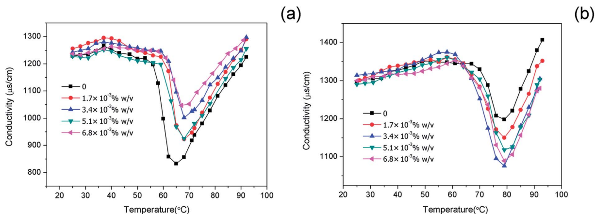
Fig. 3 Conductivity of the nanoemulsions with (a) 0.15% w/v G16-2-16, and (b) 0.20% w/v G16-2-16 at different OMT loadings as a function of temperature. The lines are used as a guide to the eye.
