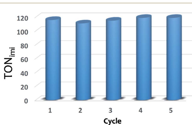
Fig. 6 Catalytic performance of XS-Sn-Imi in subsequent reaction cycles. After each cycle, the solid was washed several times with toluene and ethanol, dried and reused without additional treatments.
