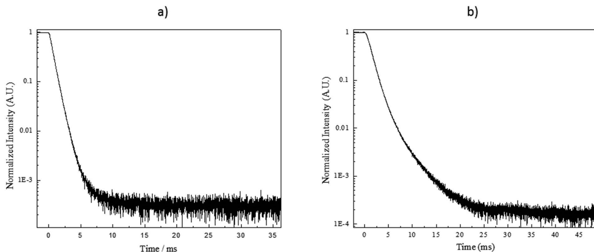
Fig. 8 Decay curves of the \text{NaF}_4\text{:Yb}^{3+},\text{Er}^{3+} particles for green (a) and red (b) emissions.
