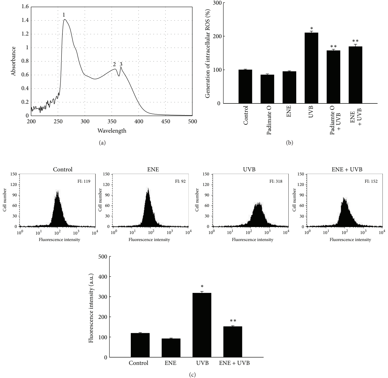
FIGURE 2: ENE absorbs UVB light and scavenges UVB-generated intracellular ROS in HaCaT keratinocytes. (a) The UV/visible spectroscopic measurement was conducted in the spectral range of 250–500 nm. Absorbance is reported in absorbance units. Peaks 1, 2, and 3 indicate peak positions at 262 nm, 356 nm, and 367 nm, respectively. (b) Intracellular ROS levels were measured using fluorescence spectrophotometry and (c) flow cytometry. *Significantly different from control cells ( P < 0.05 ); **significantly different from UVB-irradiated cells ( P < 0.05 ).
