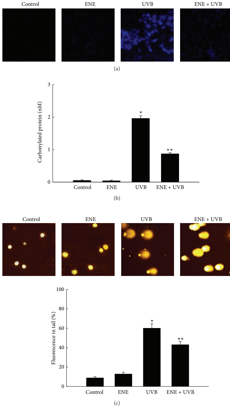
FIGURE 3: ENE protects HaCaT keratinocytes against UVB-induced lipid peroxidation, protein carbonylation, and DNA fragmentation. (a) Lipid hydroperoxide formation was detected by confocal microscopy after DPPPP staining. (b) Protein oxidation was detected by measuring the amount of protein carbonyl formation. *Significantly different from control cells ( P < 0.05 ); ** significantly different from UVB-irradiated cells ( P < 0.05 ). (c) DNA fragmentation was detected by an alkaline comet assay. *Significantly different from control cells ( P < 0.05 ); ** significantly different from UVB-irradiated cells ( P < 0.05 ).
