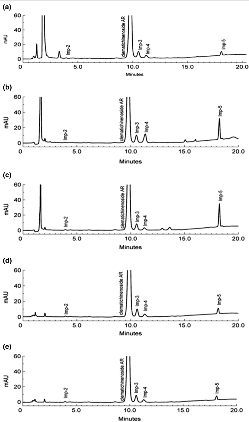
Figure 3 Typical chromatogram of clematichinenoside AR under stress conditions: (a) oxidative degradation, (b) acid hydrolysis, (c) base hydrolysis, (d) thermal degradation, (e) photolytic degradation.
