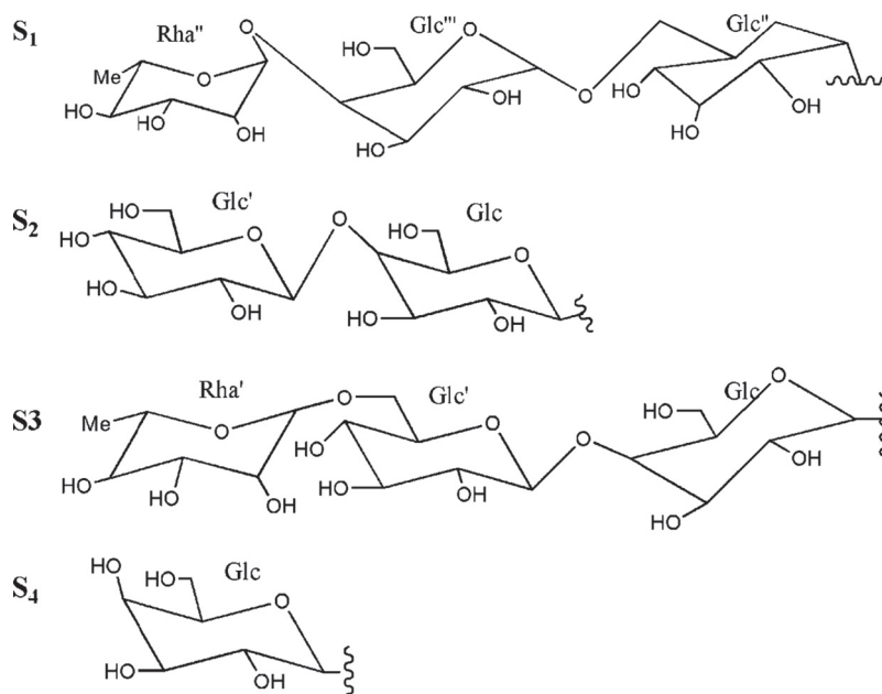
Figure 1 The chemical structures of Clematichinenoside AR and its related impurities.
